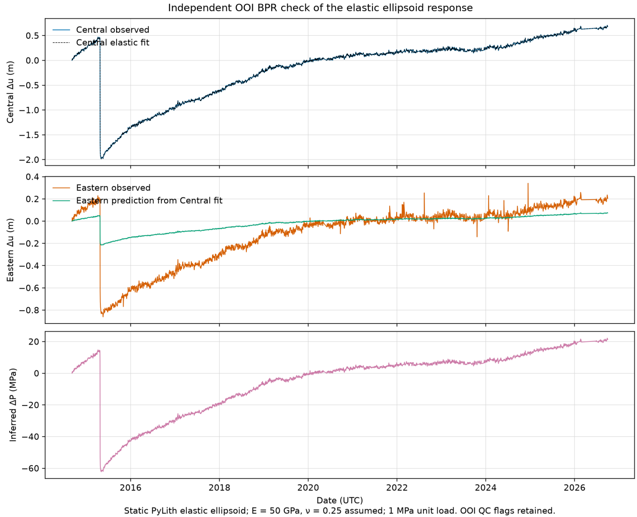
Figure 13: Static elastic ellipsoid fit to Central OOI uplift and Eastern holdout prediction. Generated by make ellipsoid-bpr-check . The amplitude mismatch and nonconverged compliance make the inferred pressure provisional.
