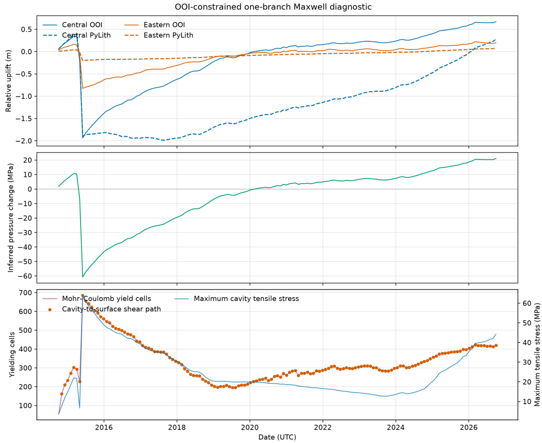
Figure 14: OOI-constrained one-branch Maxwell diagnostic. The panels compare OOI and modeled uplift, static-fit pressure, and stress-derived failure indicators. Generated by make ooi-maxwell-history-plot . Quality code 2 is retained; pressure uses static compliance; the mesh and failure assumptions remain provisional.
