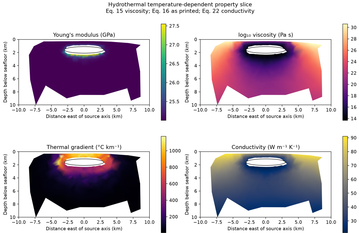
Figure 2: Hydrothermal temperature-dependent properties on a finite-thickness slice around the model y=0 plane. Cell-center values show Young’s modulus from Eq. 16 as printed, Arrhenius viscosity, the finite-element temperature gradient, and Eq. 22 conductivity. The white ellipse marks the reservoir. Side and basal temperatures extend the assumed 30 °C/km geotherm. Generated by make thermal-property-slices ; Eq. 16 remains an unresolved transcription diagnostic.
