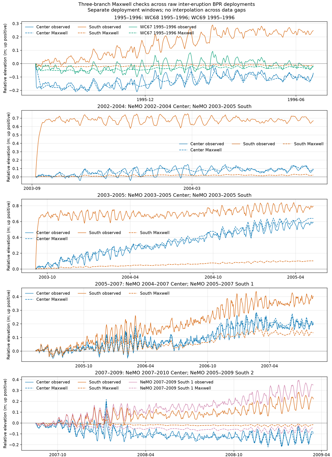
Figure 9: Three-branch Maxwell checks for raw Center/South deployment overlaps from 1995 through 2009. WC67 is held out in 1995–96 and NeMO South 1 in 2007–09. Each pair is independently zeroed; gaps are not interpolated. Generated by make reproduce .
