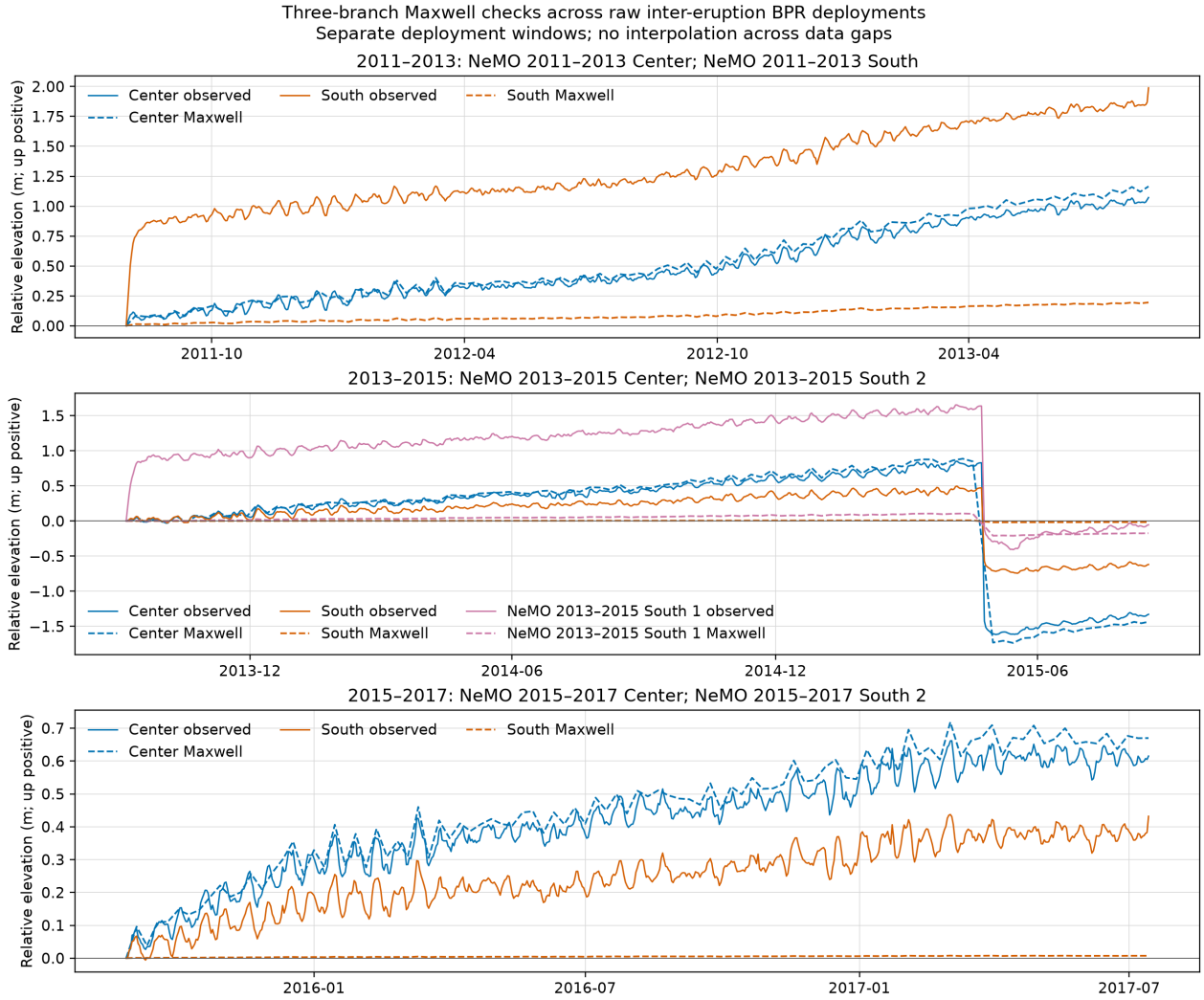
Figure 10: Three-branch Maxwell checks for raw Center/South deployment overlaps from 2011 through 2017. NeMO South 1 is held out for 2013–15. Each pair is independently zeroed; gaps are not interpolated. Center pressure uses static elastic compliance, and synthetic branch parameters and uncorrected records are diagnostic assumptions. The MGDS channels are original RawDep data from IEDA/322282, distributed under CC BY-NC-SA 3.0. Generated by make reproduce .
