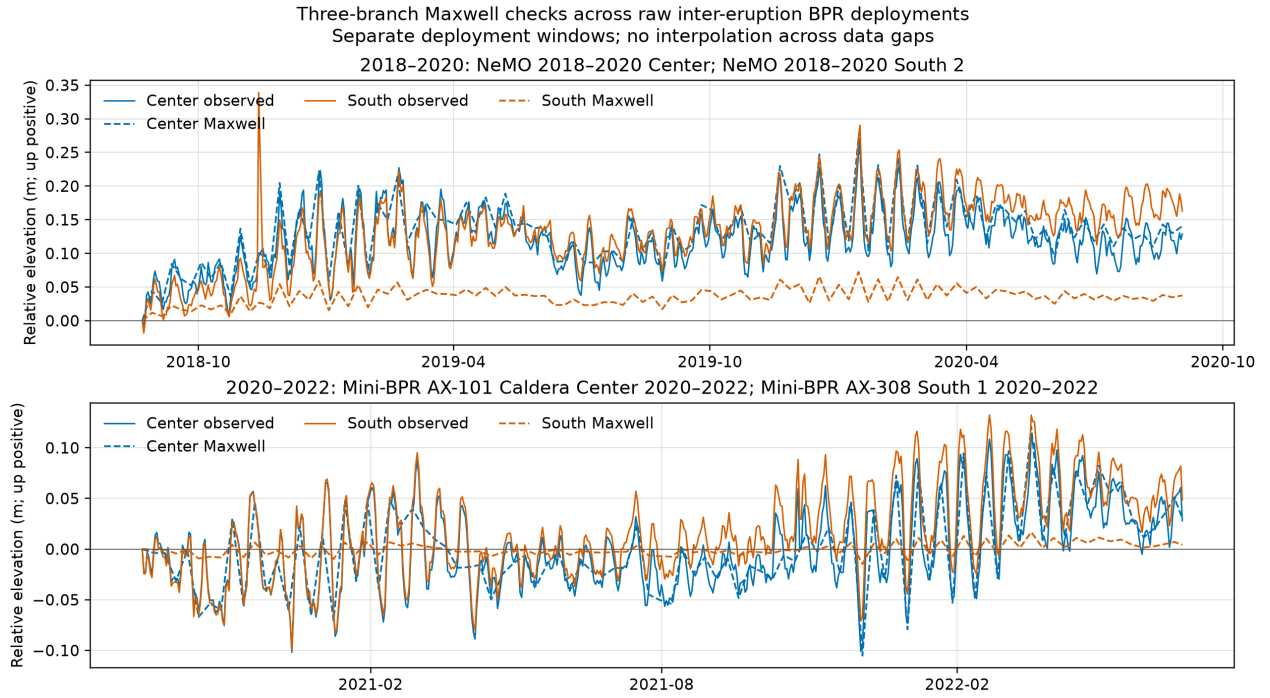
Figure 11: Three-branch Maxwell checks for original raw Center/South deployments from 2018 through 2022. The upper panel uses the 15-second moored-BPR RawDep channels; the lower panel uses the 100-second miniBPR RawDepth(m) channels. Each pair is independently zeroed, with no pressure-drift or tide correction. Generated by make_historical-post-2017-bpr-check .
