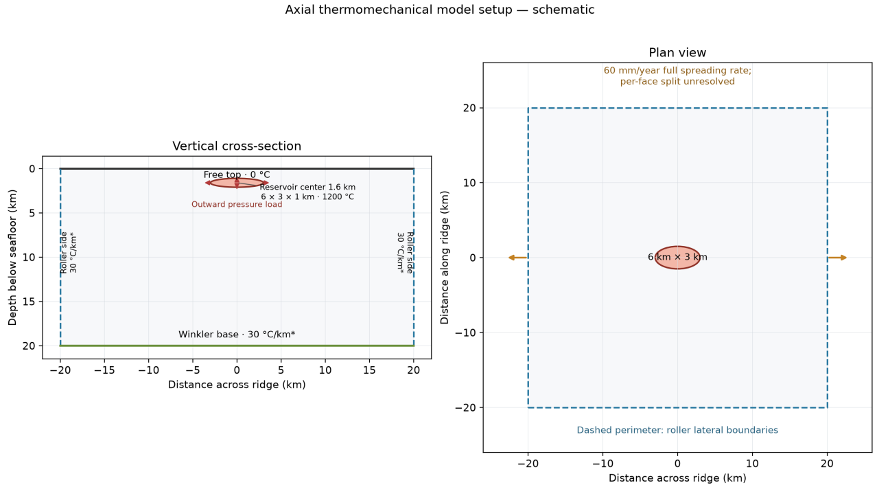
The 40 × 40 × 20 km box is a project fallback; the written model extent is unavailable. *The side and basal 30 °C/km geotherm is an explicit thermal assumption. Reservoir depth is 1.6 km to center; Winkler stiffness and the tectonic face-rate split are unresolved.
