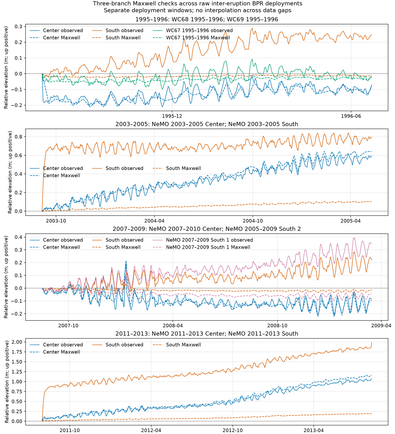
Figure 6: Three-branch Maxwell checks for four raw Center/South deployment overlaps from 1995 through 2013, with WC67 added to the 1995–96 panel and NeMO South 1 added to the 2007–09 panel as held-out raw BPR stations. Each deployment pair is independently zeroed; gaps are not interpolated. Center pressure uses static elastic compliance, and the synthetic branch parameters and uncorrected records are diagnostic assumptions. Generated by make historical-generalized-maxwell-check .
