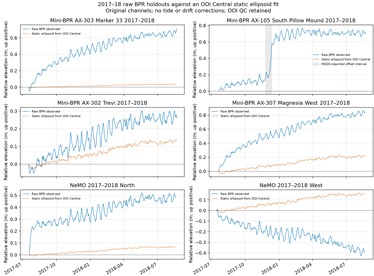
Figure 12: Original MGDS 2017–18 raw BPR holdouts and static ellipsoid predictions scaled from OOI Central. The first shared date sets each series baseline; the shaded AX-105 interval is excluded from its primary metrics. OOI quality codes are retained and no tide or drift corrections are applied. Generated by make historical-ooi-bpr-holdouts .
