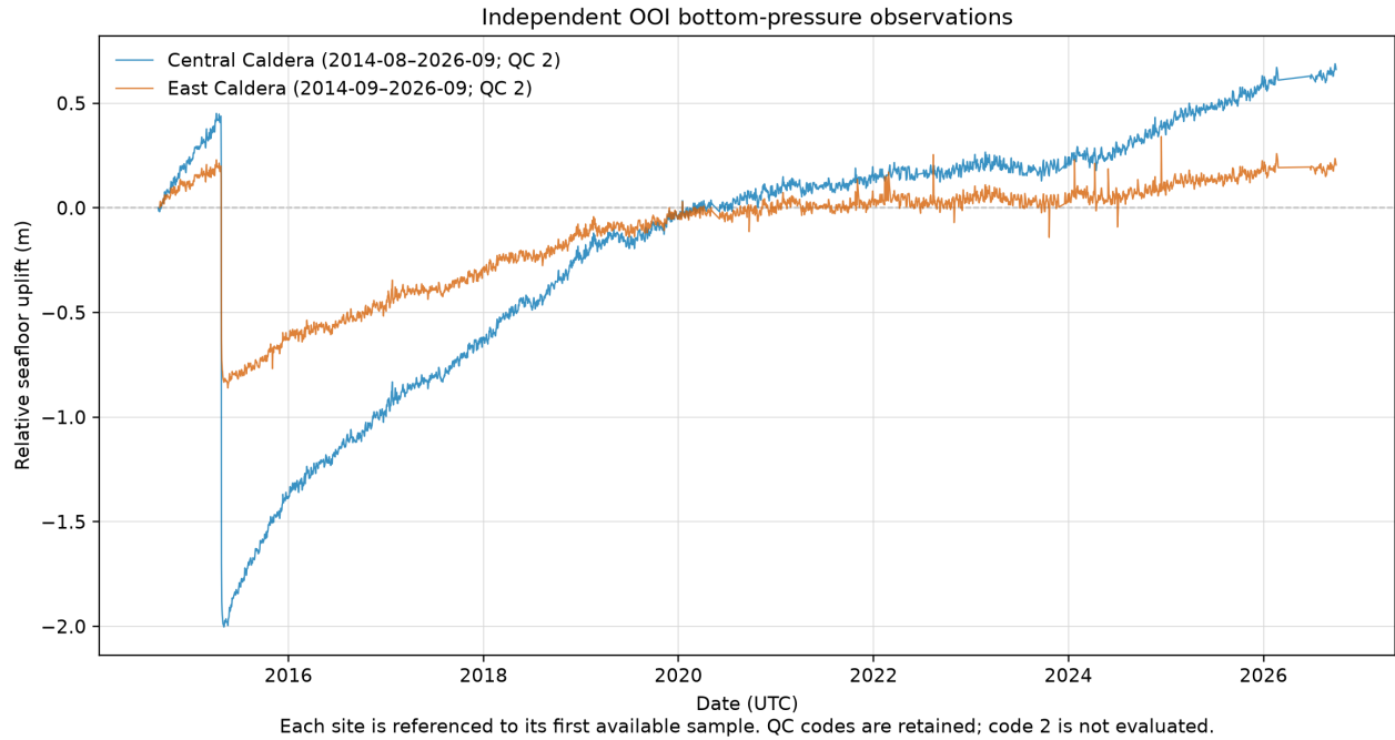
Figure 6: Daily OOI relative uplift at Central and Eastern Caldera from each site’s first available record. Generated by make bpr-observation-plot ; aggregate quality code 2 (NOT EVALUATED) is retained. The data show the observed interval available for independent model checking.
