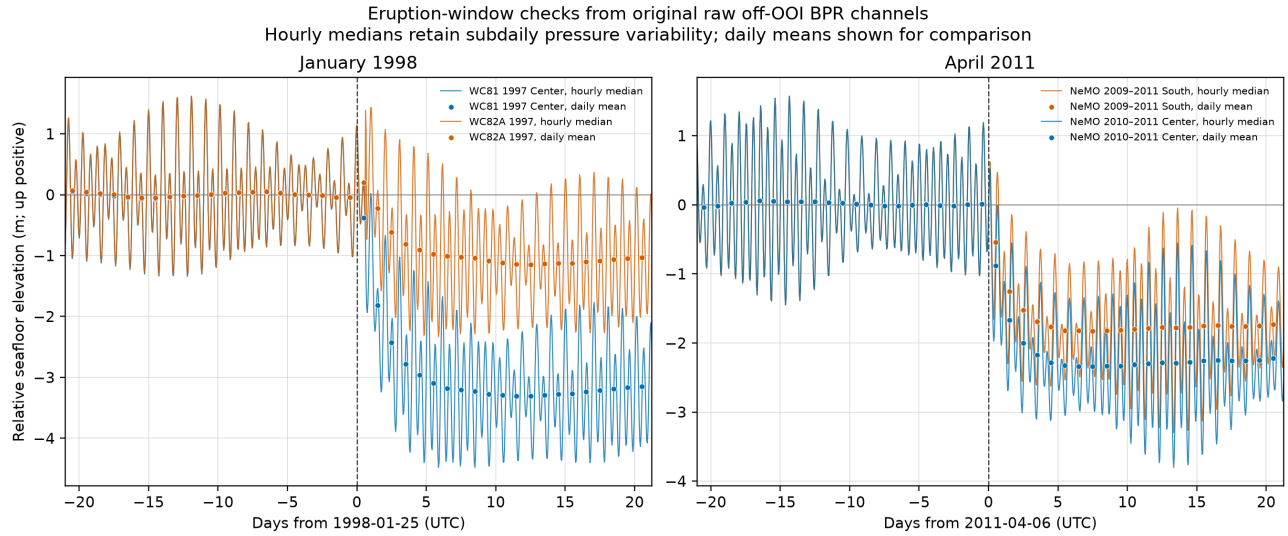
Figure 21: Hourly medians and daily means from original raw off-OOI BPR channels around the 1998 and 2011 events. Each station has its own baseline from days -7 through -1 ; hours require 75 percent sample coverage. No tidal, oceanographic, filter, or drift correction is applied. Vertical markers show the event date at day-level resolution and do not estimate an eruption time. Generated by make_historical-bpr-subdaily-event-check from raw NOAA/NCEI dbar and MGDS RawDep/Depth channels. Sources: NOAA/NCEI (doi:10.7289/V5F18WNS) and original MGDS IEDA/322282 channels (William Chadwick, Scott Nooner, and MGDS; CC BY-NC-SA 3.0).
