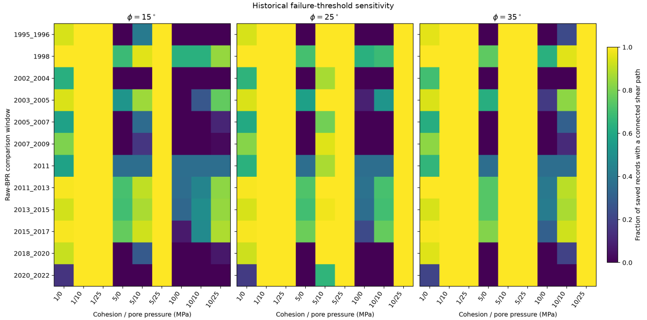
Figure 8: Fraction of saved records with a connected cavity-to-top shear path across a diagnostic grid of cohesion and pore pressure, shown for three direct friction angles. Zero-valued cells have no path in any saved record. The grid postprocesses independently generated raw-BPR-driven PyLith stress histories and does not assign tensile strength or calibrate rock properties. Generated by make historical-failure-threshold-sensitivity .
