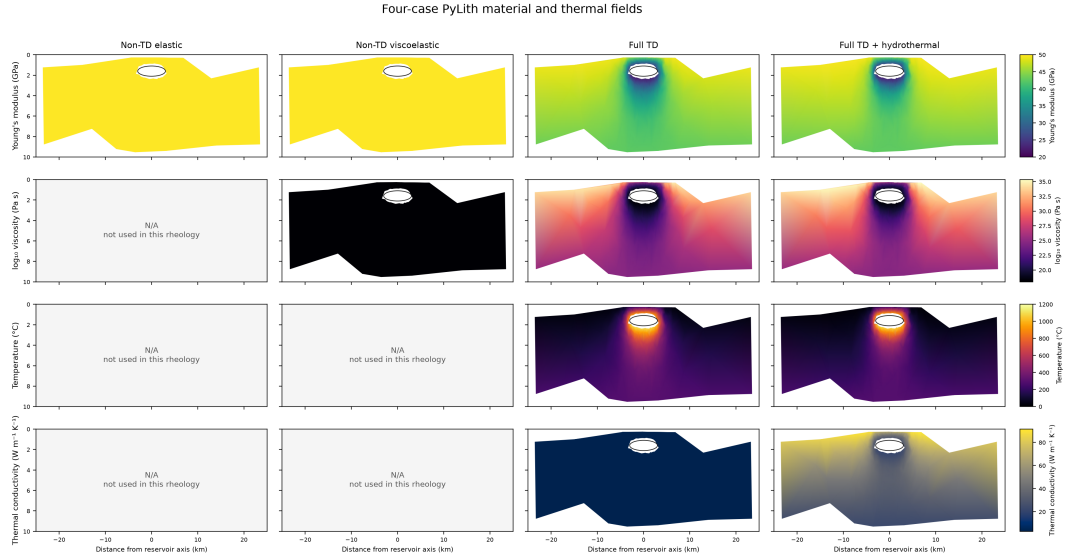
Figure 3: Project-generated four-case property matrix in the requested 4 by 4 layout. Rows show Young's modulus, log viscosity, temperature, and thermal conductivity; columns are non-temperature-dependent elastic, non-temperature-dependent viscoelastic, Full TD, and Full TD plus hydrothermal cases. The 50-to-20 GPa modulus mapping follows the project instruction, while Maxwell branch viscosities are synthetic. The maps cover the project-directed 50 by 50 km horizontal box and 0–10 km depth. These are PyLith property fields used by the bounded common 1 MPa, two-year diagnostic run, not Cabaniss output or a calibrated eruption prediction. The solve uses a fixed base pending a validated Axial Winkler foundation. Generated by make figure3-rheology-properties .
