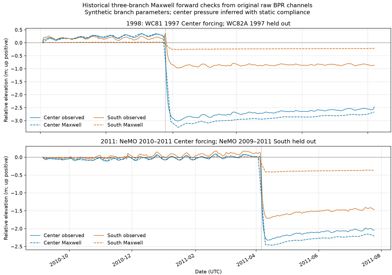
Figure 9: Three-branch generalized Maxwell forward checks against raw daily BPR observations for the 1998 and 2011 Center/South deployment pairs. Center pressure is inferred from static elastic compliance; South is held out. Synthetic branch properties, first-common-day zeroing, uncorrected raw records, and nonconverged compliance limit interpretation. Generated by make historical-generalized-maxwell-check .
