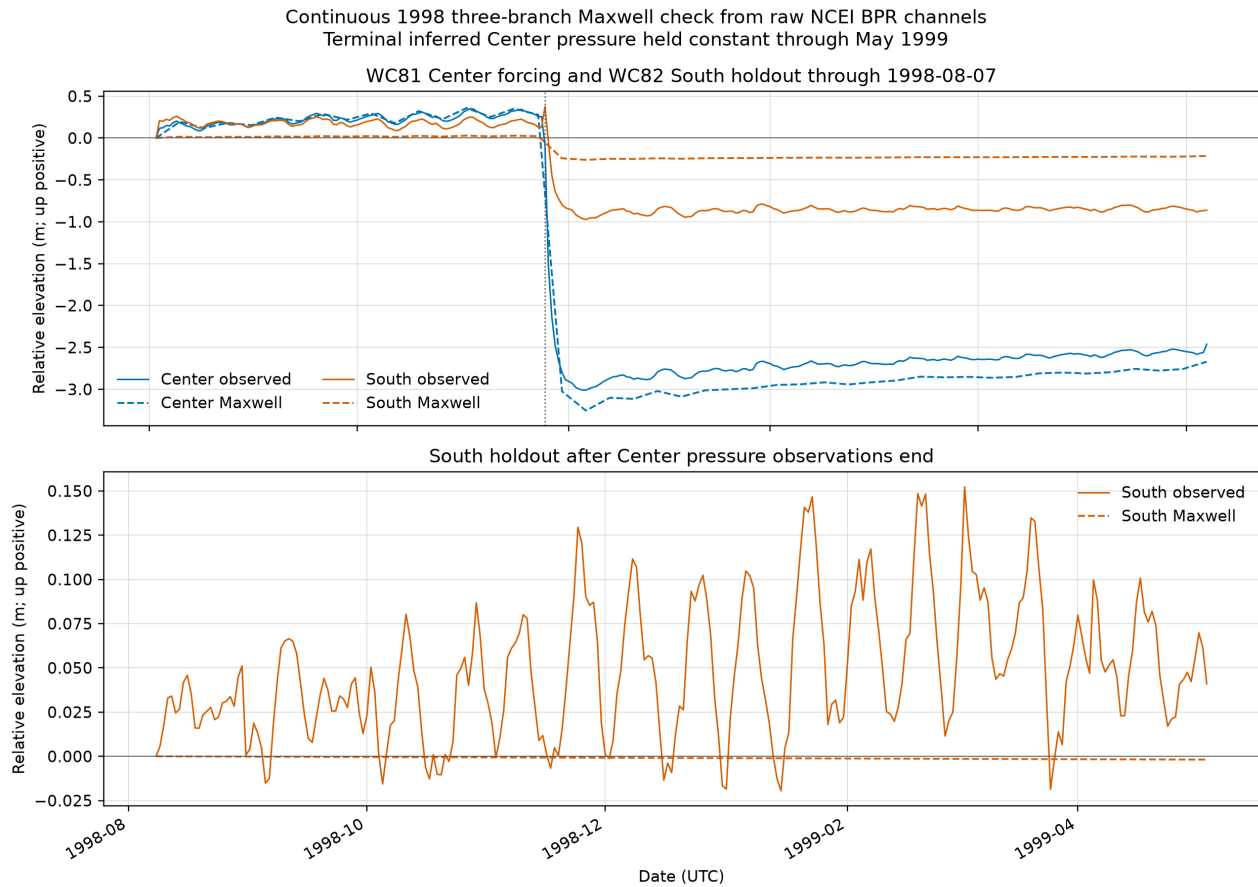
Figure 11: Continuous 1998 three-branch Maxwell check using only original NCEI WC81 Center and WC82 South absolute-pressure channels. The upper panel compares Center forcing and the event South holdout through 7 August 1998; the lower panel checks the South station through 4 May 1999 after Center pressure observations end. The two WC82 South files are aligned from their eight-day raw overlap. Terminal inferred Center pressure is held constant for 270 days. Synthetic branch parameters, raw ocean variability, and nonconverged compliance limit interpretation. Source: NCEI DART raw BPR archive, doi:10.7289/V5F18WNS. Generated by make historical-generalized-maxwell-1998-continuous-check .
