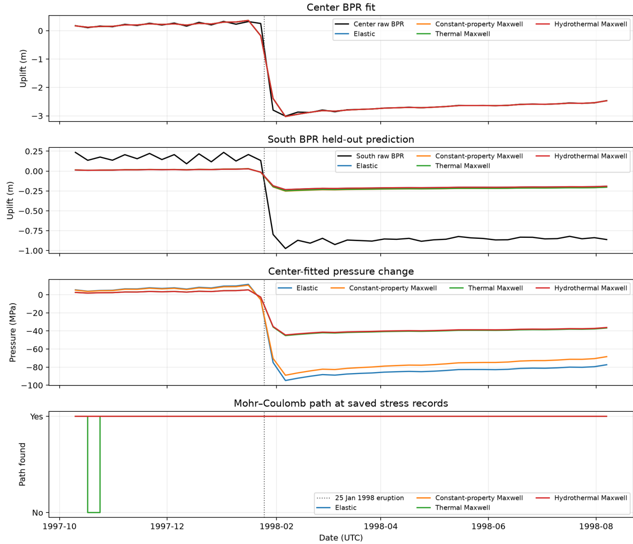
Figure 22: Four pressure calibrations against original raw NCEI WC81 Center data, with WC82A South held out and provisional connected-path states shown at saved stress records. The dotted line marks the observed 25 January 1998 eruption. Each pressure history is fitted independently, and Center includes the eruption deflation and later records. Synthetic branch parameters, the nonconverged mesh, and unresolved failure assumptions make this a retrospective diagnostic. No MGDS Fox duplicate or Cabaniss-associated data products were used. Generated by make historical-four-case-bpr-calibration .
