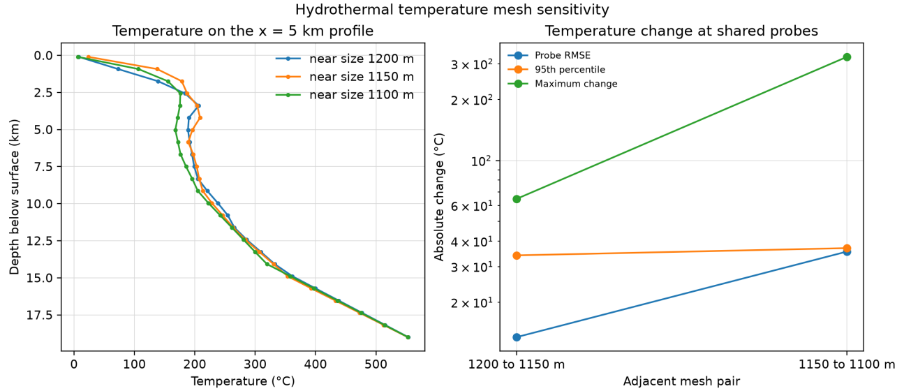
Figure 5: Hydrothermal temperature sensitivity across three bounded tetrahedral meshes. The left panel shows interpolated temperatures along a common vertical profile. The right panel shows RMSE, 95th-percentile, and maximum absolute changes across 105 common host-rock probes for adjacent meshes. Meshes are independently generated and non-nested; the probe changes diagnose spatial sensitivity but do not establish convergence. Generated by make thermal-mesh-sensitivity .
