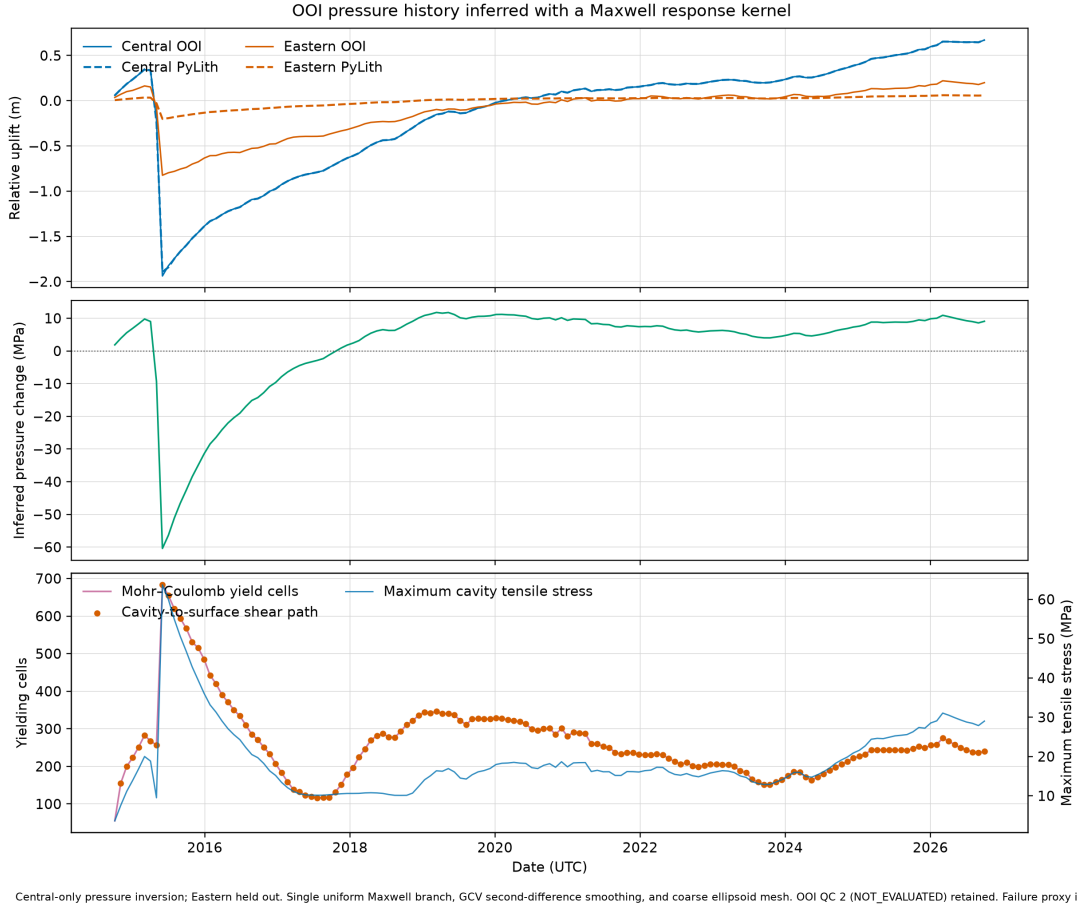
Figure 19: OOI Central pressure inversion with a one-branch Maxwell response kernel. Central is fitted and Eastern is held out; dashed curves show the direct PyLith history. The plot includes the inferred pressure and provisional failure diagnostics. Generated by make ooi-maxwell-pressure-inversion from independent OOI records. The smoothness prior, pressure scale, and nonconverged mesh remain provisional.
