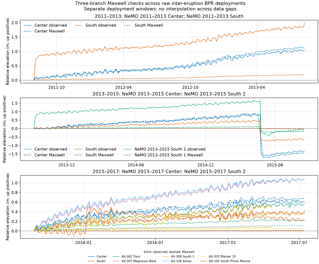
Figure 14: Three-branch Maxwell checks for raw Center/South deployment overlaps from 2011 through 2017. NeMO South 1 is held out for 2013–15. Each pair is independently zeroed; gaps are not interpolated. Center pressure uses static elastic compliance, and synthetic branch parameters and uncorrected records are diagnostic assumptions. The MGDS channels are original RawDep data from IEDA/322282, distributed under CC BY-NC-SA 3.0. Generated by make reproduce .
