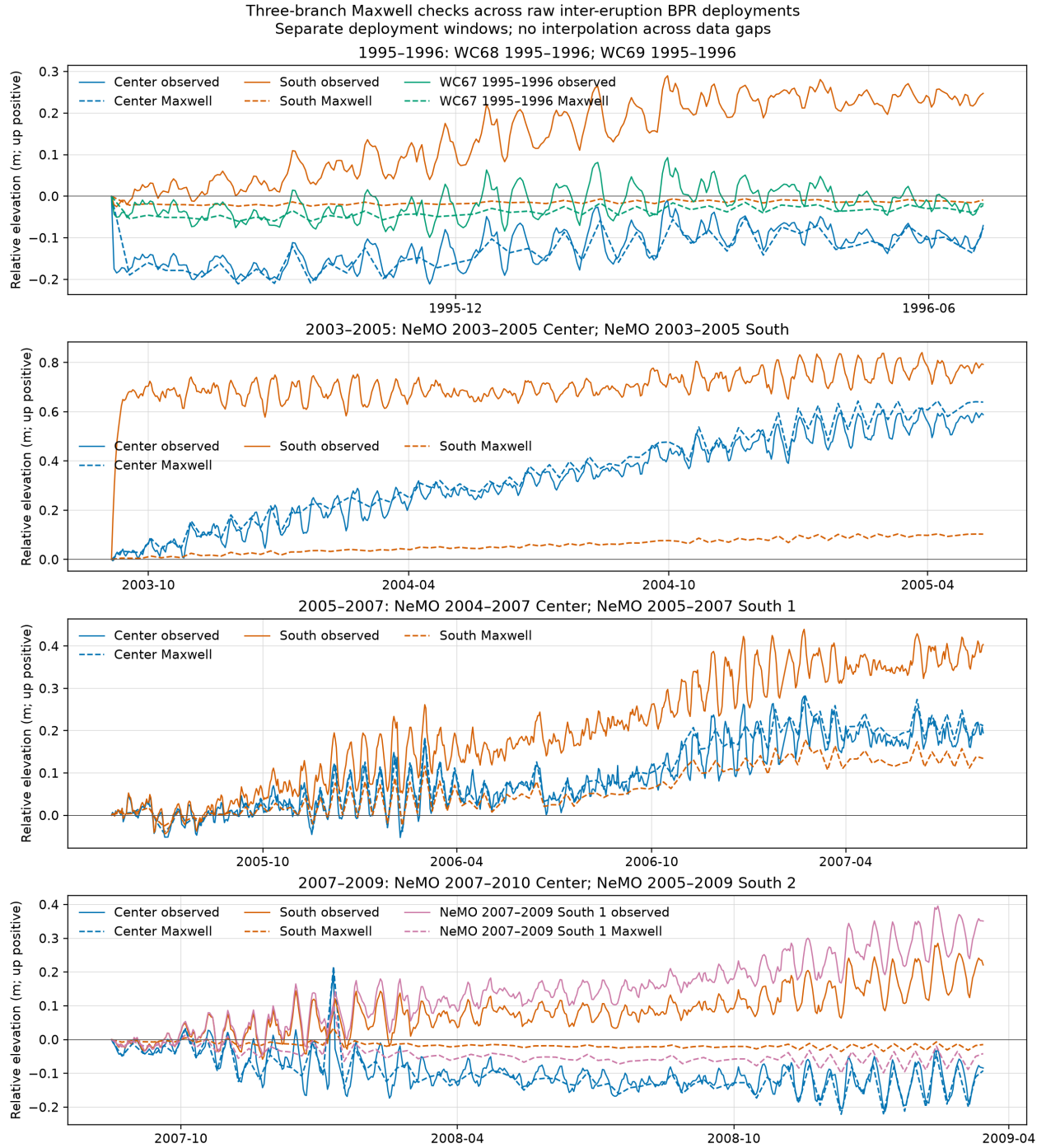
Figure 8: Three-branch Maxwell checks for raw Center/South deployment overlaps from 1995 through 2009. WC67 is held out in 1995–96 and NeMO South 1 in 2007–09. Each pair is independently zeroed; gaps are not interpolated. Generated by make reproduce .
