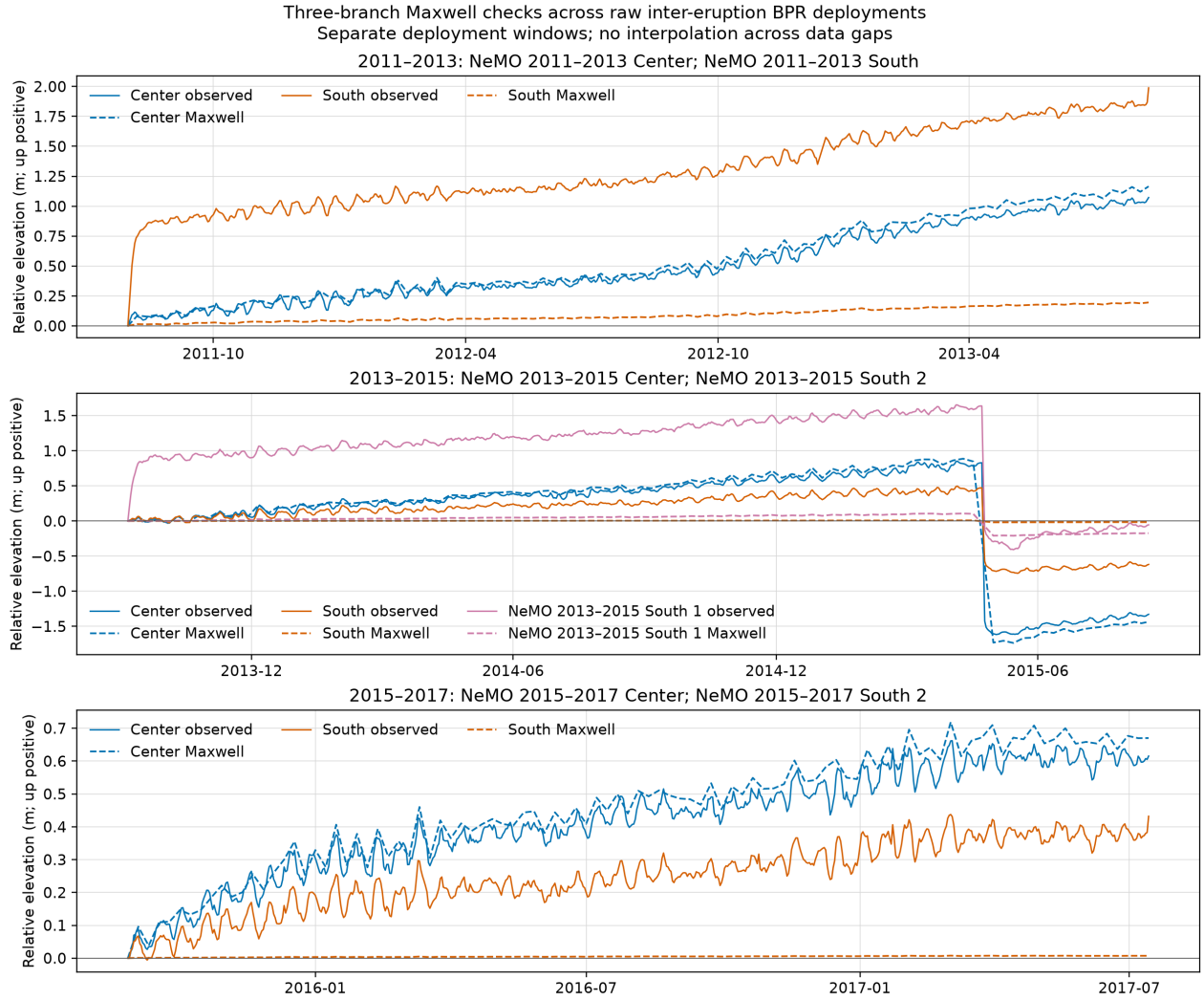
Figure 9: Three-branch Maxwell checks for raw Center/South deployment overlaps from 2011 through 2017. NeMO South 1 is held out for 2013–15. Each pair is independently zeroed; gaps are not interpolated. Center pressure uses static elastic compliance, and synthetic branch parameters and uncorrected records are diagnostic assumptions. The MGDS channels are original RawDep data from IEDA/322282, distributed under CC BY-NC-SA 3.0. Generated by make reproduce .
