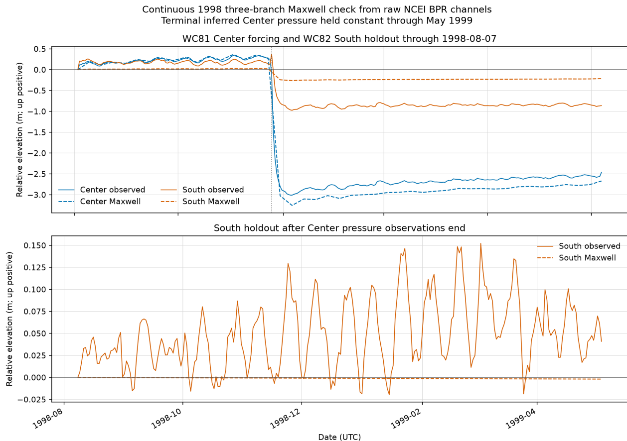
Figure 7: Continuous 1998 three-branch Maxwell check using only original NCEI WC81 Center and WC82 South absolute-pressure channels. The upper panel compares Center forcing and the event South holdout through 7 August 1998; the lower panel checks the South station through 4 May 1999 after Center pressure observations end. The two WC82 South files are aligned from their eight-day raw overlap. Terminal inferred Center pressure is held constant for 270 days. Synthetic branch parameters, raw ocean variability, and nonconverged compliance limit interpretation. Source: NCEI DART raw BPR archive, doi:10.7289/V5F18WNS. Generated by make historical-generalized-maxwell-1998-continuous-check .
