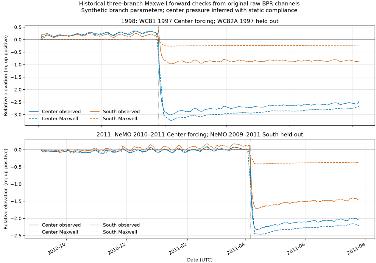
Figure 5: Three-branch generalized Maxwell forward checks against raw daily BPR observations for the 1998 and 2011 Center/South deployment pairs. Center pressure is inferred from static elastic compliance; South is held out. Synthetic branch properties, first-common-day zeroing, uncorrected raw records, and nonconverged compliance limit interpretation. Generated by make historical-generalized-maxwell-check .
