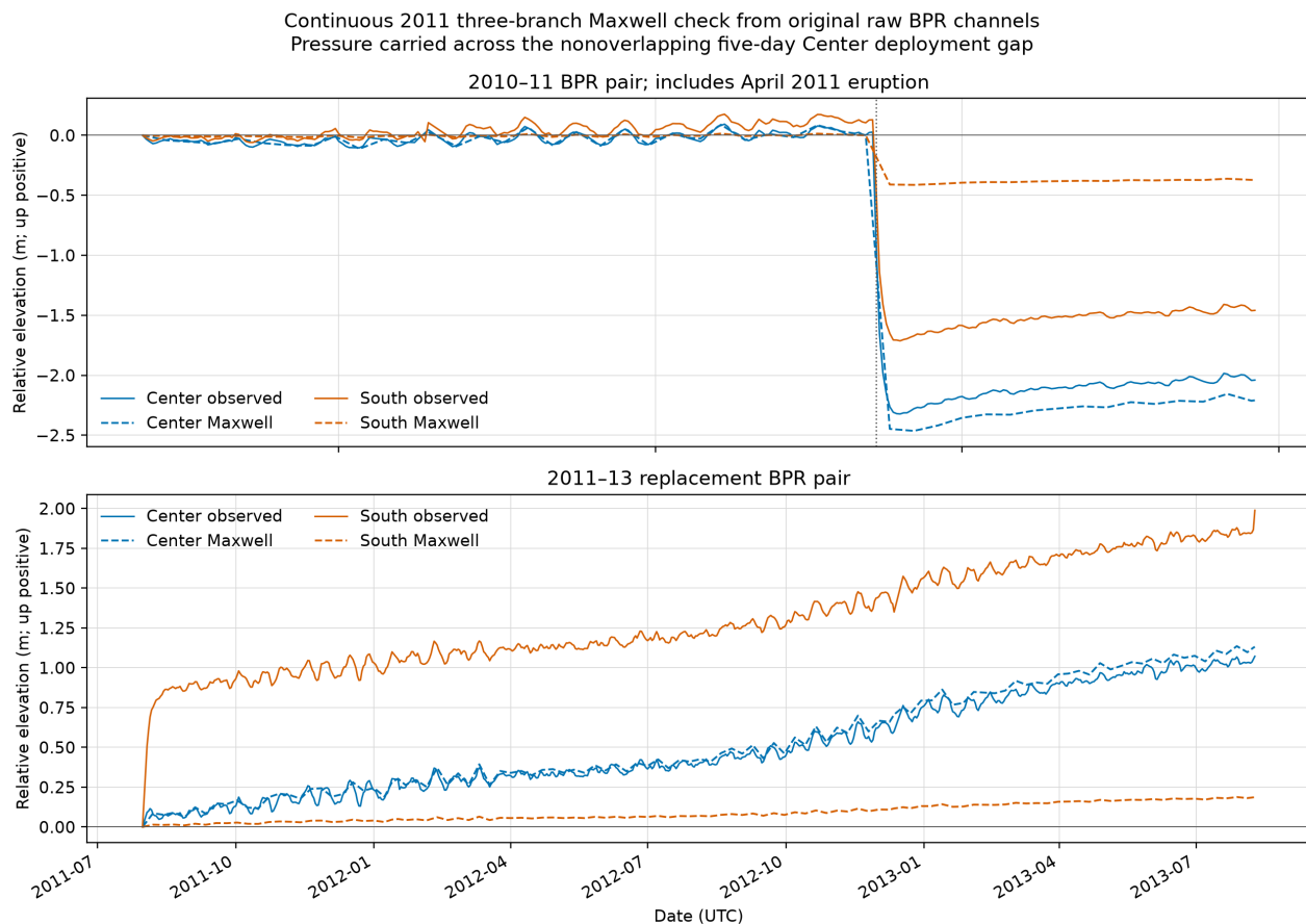
Figure 6: Continuous 2011 three-branch Maxwell check from original raw MGDS BPR channels. Each panel shows Center-forced predictions and its paired South holdout, independently baselined by deployment. The Center pressure series are joined across a five-day gap by holding the final pressure constant. The eruption date is marked in the upper panel. Synthetic branch parameters, raw instrument effects, and nonconverged compliance limit interpretation. Source channels: MGDS IEDA/322282 (Chadwick et al., 2023), CC BY-NC-SA 3.0. Generated by make historical-generalized-maxwell-2011-continuous-check .
