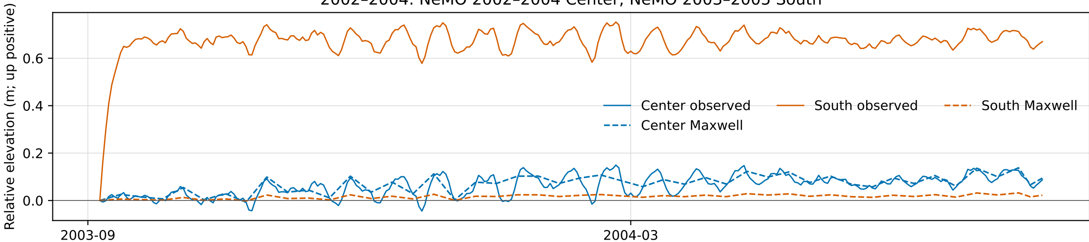
Three-branch Maxwell checks across raw inter-eruption BPR deployments Separate deployment windows; no interpolation across data gaps 2002-2004: NeMO 2002-2004 Center; NeMO 2003-2005 South
