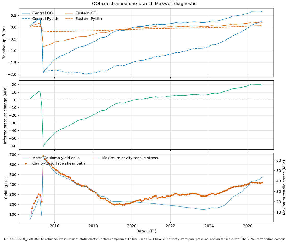
Figure 8: OOI-constrained one-branch Maxwell diagnostic. The panels compare OOI and modeled uplift, static-fit pressure, and stress-derived failure indicators. Generated by make ooi-maxwell-history-plot . Quality code 2 is retained; pressure uses static compliance; the mesh and failure assumptions remain provisional.
