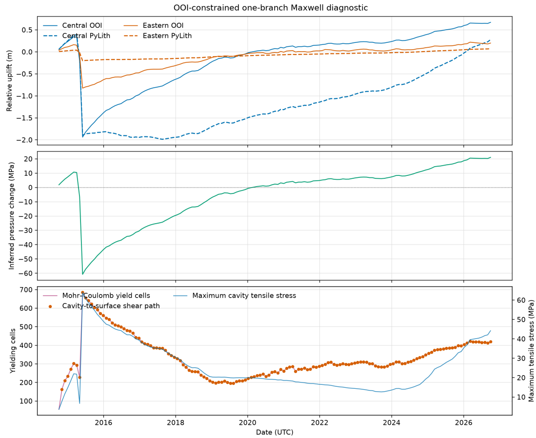
Figure 11: OOI-constrained one-branch Maxwell diagnostic. The panels compare OOI and modeled uplift, static-fit pressure, and stress-derived failure indicators. Generated by make ooi-maxwell-history-plot . Quality code 2 is retained; pressure uses static compliance; the mesh and failure assumptions remain provisional.
