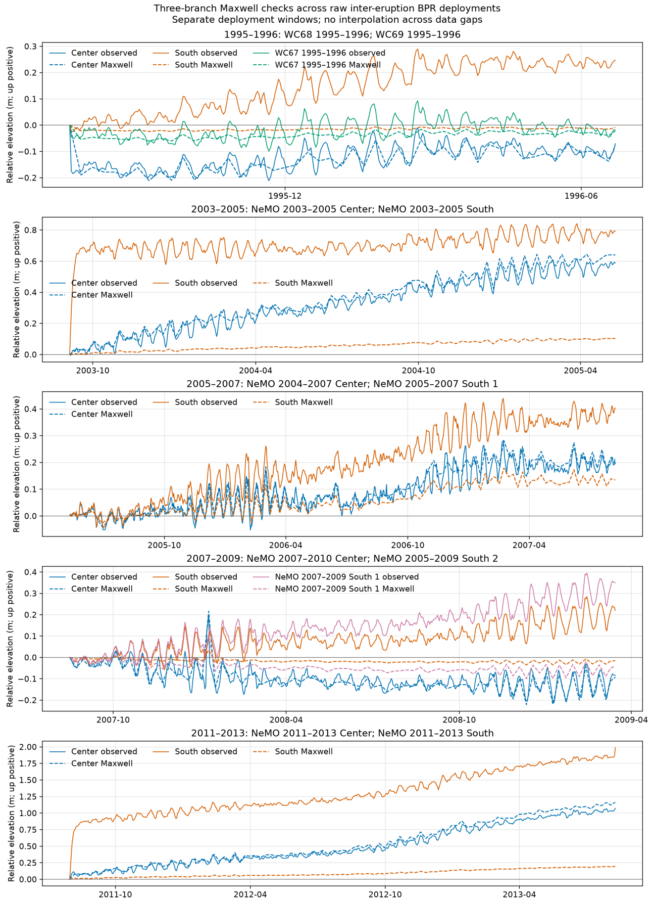
Figure 8: Three-branch Maxwell checks for five raw Center/South deployment overlaps from 1995 through 2013, with WC67 added to the 1995–96 panel and NeMO South 1 added to the 2007–09 panel as held-out raw BPR stations. Each deployment pair is independently zeroed; gaps are not interpolated. Center pressure uses static elastic compliance, and the synthetic branch parameters and uncorrected
