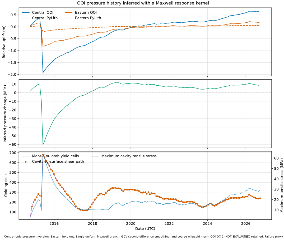
Figure 12: OOI Central pressure inversion with a one-branch Maxwell response kernel. Central is fitted and Eastern is held out; dashed curves show the direct PyLith history. The plot includes the inferred pressure and provisional failure diagnostics. Generated by make ooi-maxwell-pressure-inversion from independent OOI records. The smoothness prior, pressure scale, and nonconverged mesh remain provisional.
