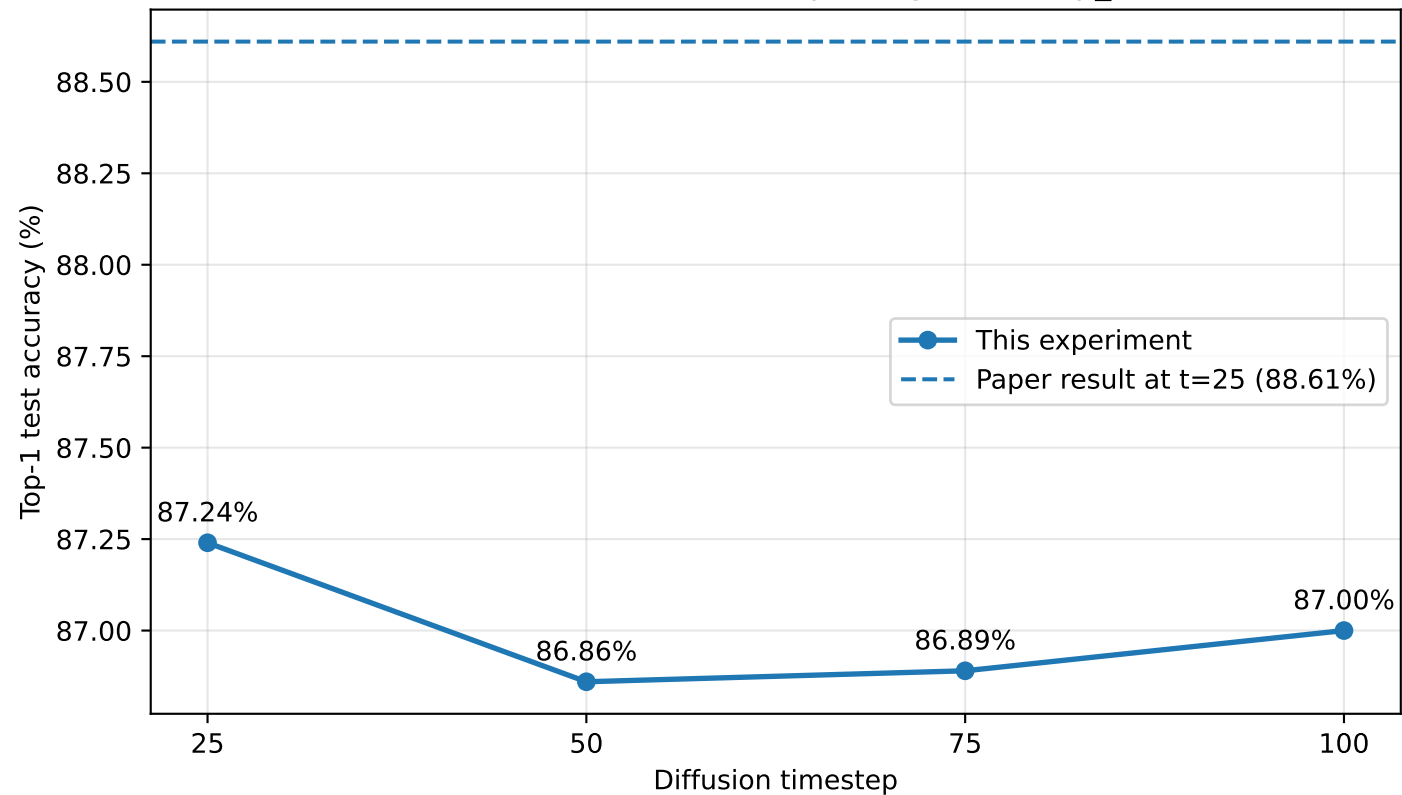
Effect of diffusion timestep using SD-1.5 up_ft1
