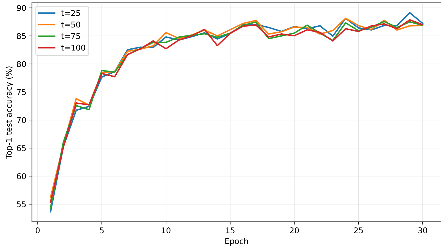
Diff-C test accuracy during training
