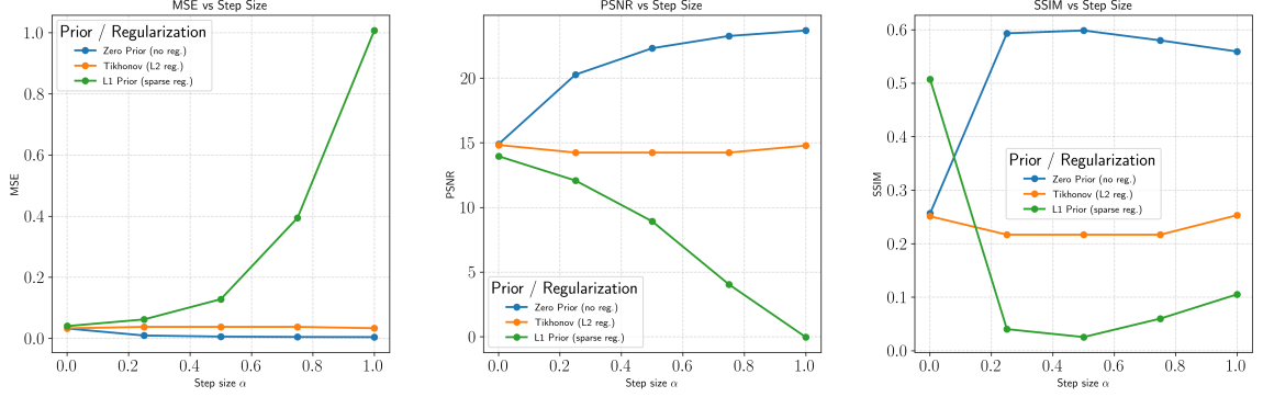
Fig. 5. Hyperparameters comparison: MSE (left), PSNR (center), and SSIM (right).
