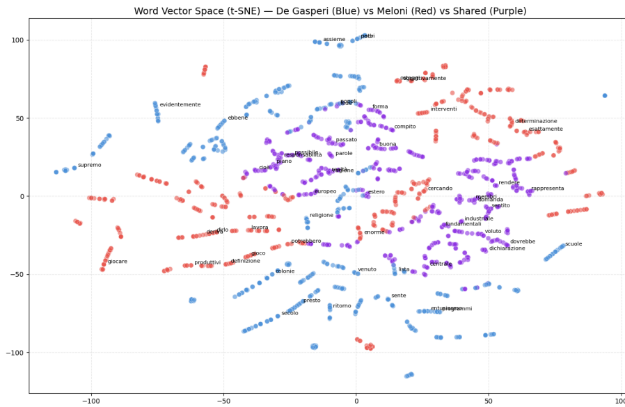
Fig. 2. t-SNE for top-1000 words for both PMs. In red Meloni-only words, in blue De Gasperi-only words, and in purple shared words.
