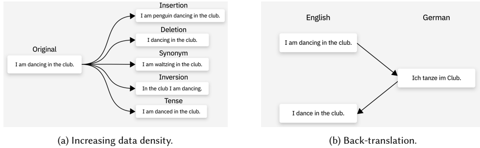
Fig. 1. Data augmentation techniques, such as synonym replacement and back-translation. Source: Kavlakoglu, IBM [21].
