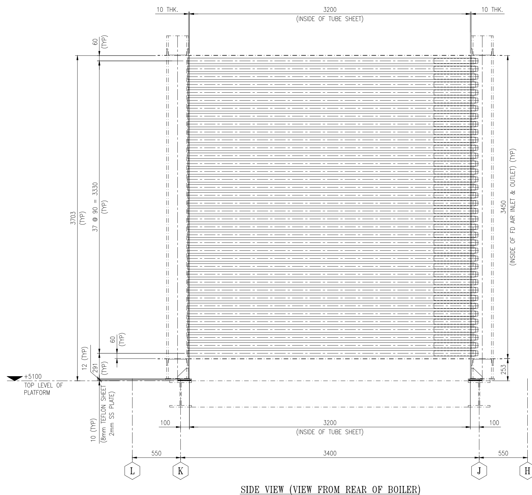
SIDE VIEW (VIEW FROM REAR OF BOILER)
