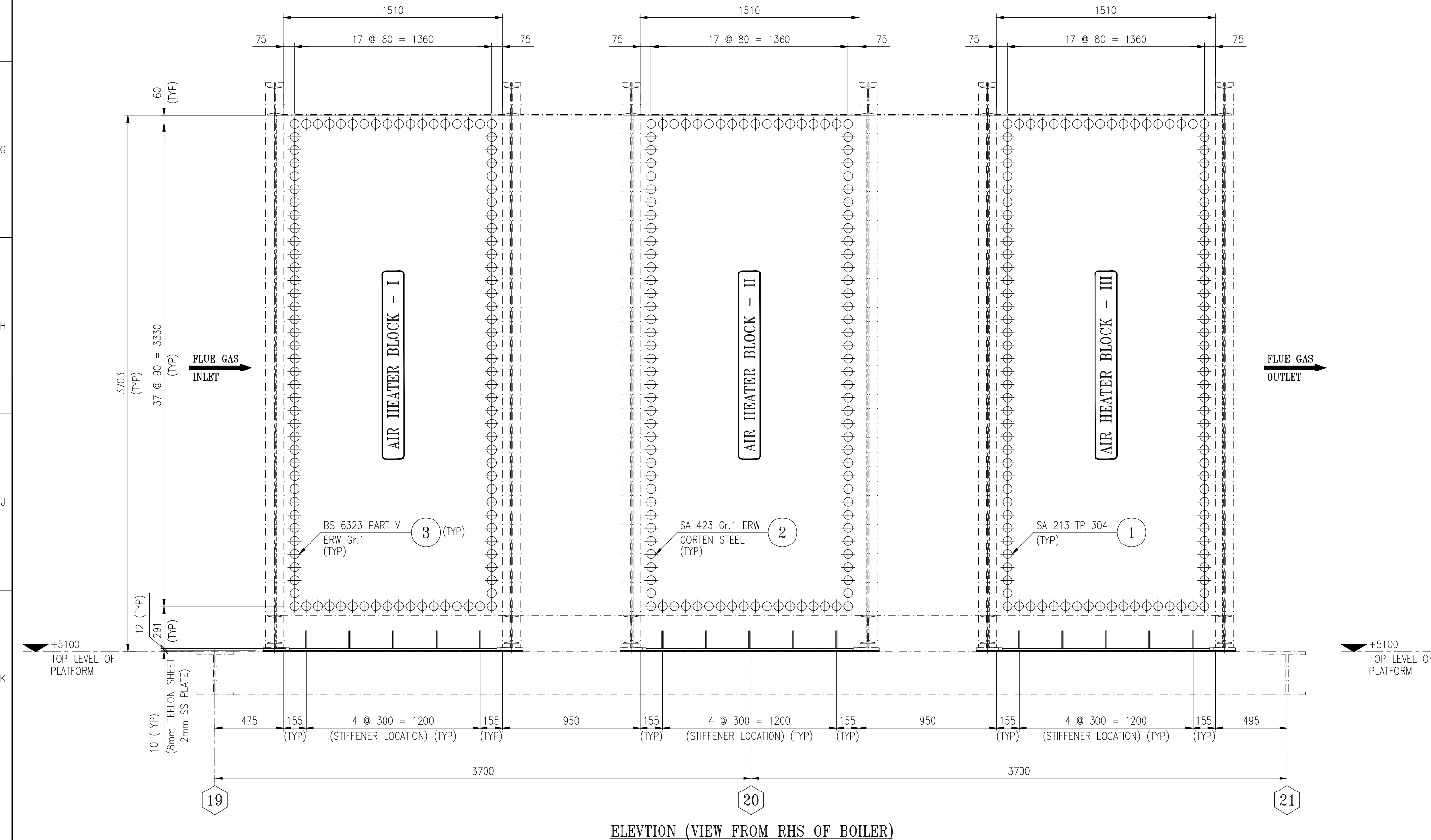
ELEVATION (VIEW FROM RHS OF BOILER)
