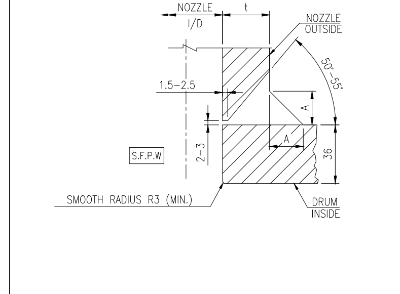
WELD DETAIL OF NOZZLE TO DRUM [FOR MARK Nos. N16,N18/1,N18/2,N20 TO N31,N38,N39/1,N39/2 & N40]
