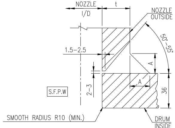
WELD DETAIL OF NOZZLE TO DRUM [FOR MARK Nos. N1 & N2]
