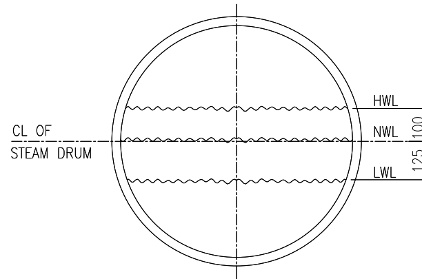
WATER LEVELS FOR STEAM DRUM
