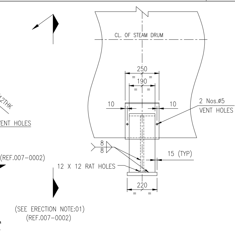
WELD DETAIL OF NOZZLE TO DRUM [FOR MARK No. N4]
