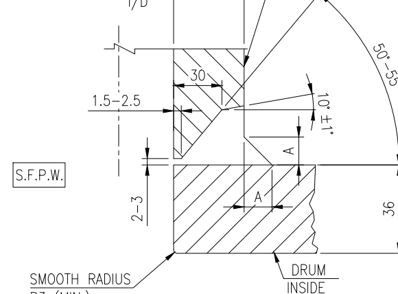
WELD DETAIL OF NOZZLE TO DRUM [FOR MARK No. N4]
