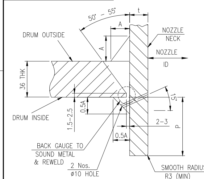
WELD DETAIL OF NOZZLE TO DRUM MARK Nos. N14/1 & N14/2
