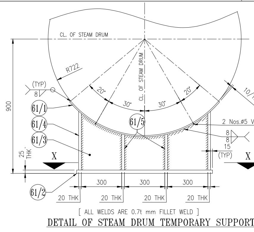
DETAIL OF STEAM DRUM TEMPORARY SUPPORT
