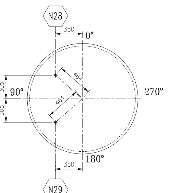
DETAIL OF STEAM DRUM DISHED END PIPE NOZZLES (TYP. FOR RHS)
