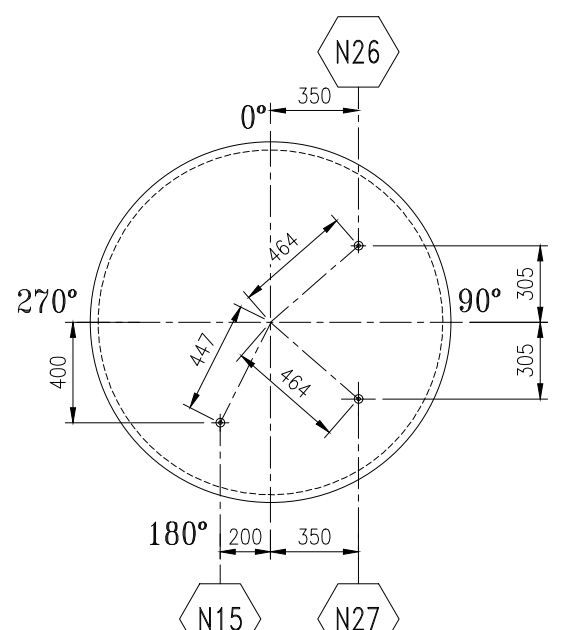
DETAIL OF STEAM DRUM DISHED END PIPE NOZZLES (TYP. FOR LHS)
