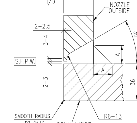
WELD DETAIL OF NOZZLE TO DRUM [FOR MARK Nos. N5/1 TO N5/6, N6/1 TO N6/5 & N9]
