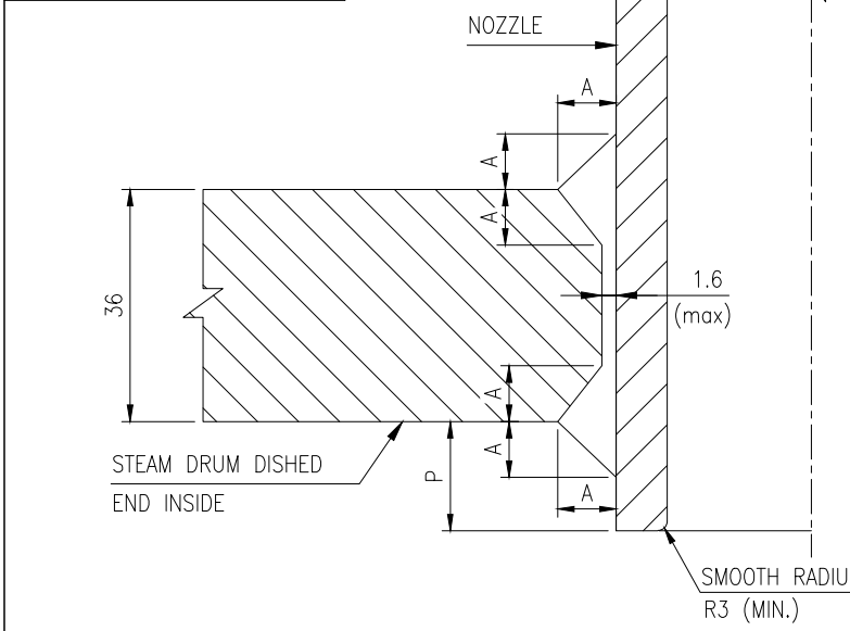
WELD DETAIL OF NOZZLE TO DRUM [FOR MARK No. N15]
