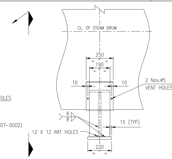
(SEE ERECTION NOTE:01) (REF.007-0002)
