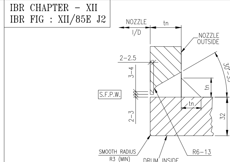
WELD DETAIL OF NOZZLE TO DRUM [FOR MARK Nos. N4/1, N4/2, N5/1 TO N5/8 N6/1 TO N6/6 & N9]
