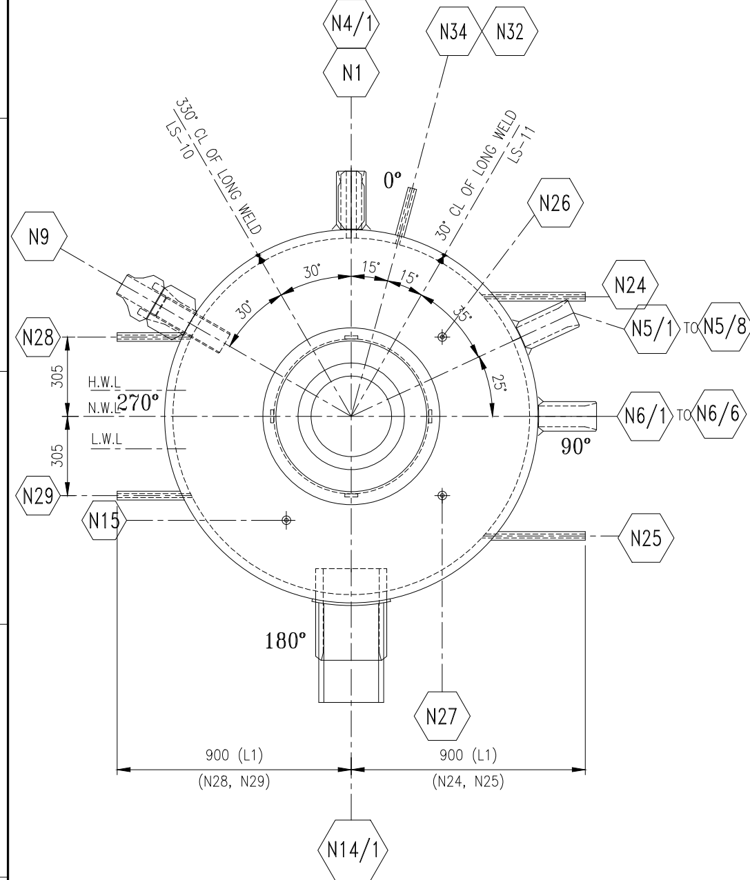
VIEW - AA (LHS OF BOILER)
