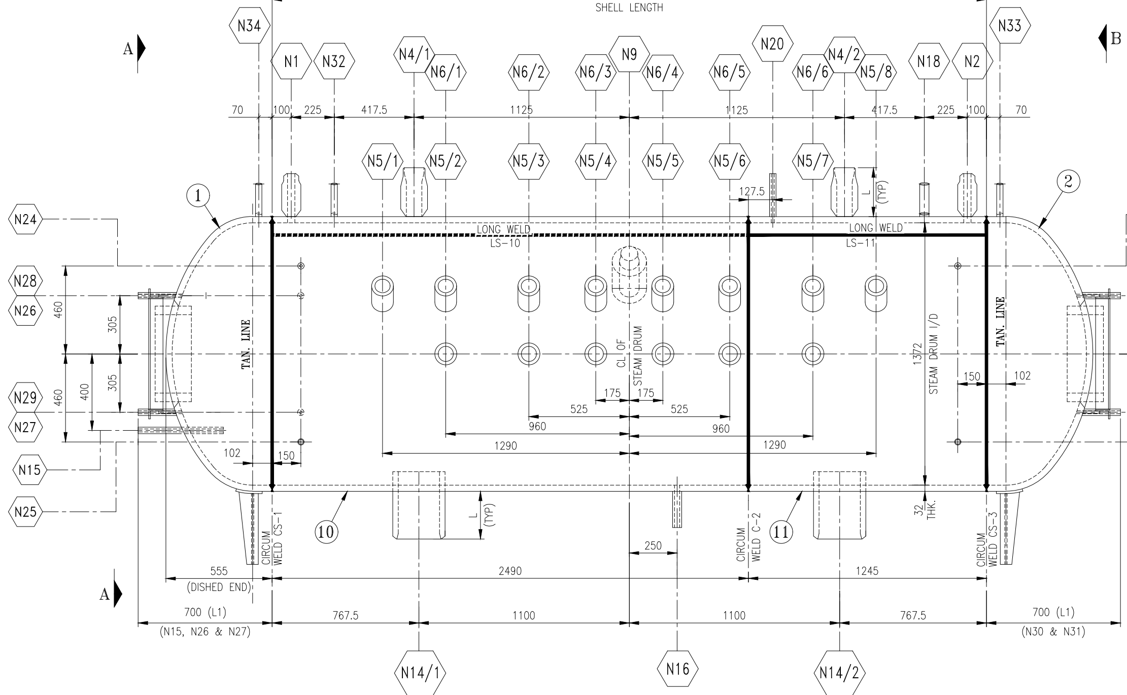
ELEVATION (VIEWED FROM FRONT OF BOILER) ARRANGEMENT OF STEAM DRUM
