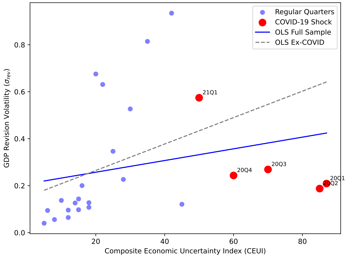
Influence of Economic Turbulence on Predictive Errors
