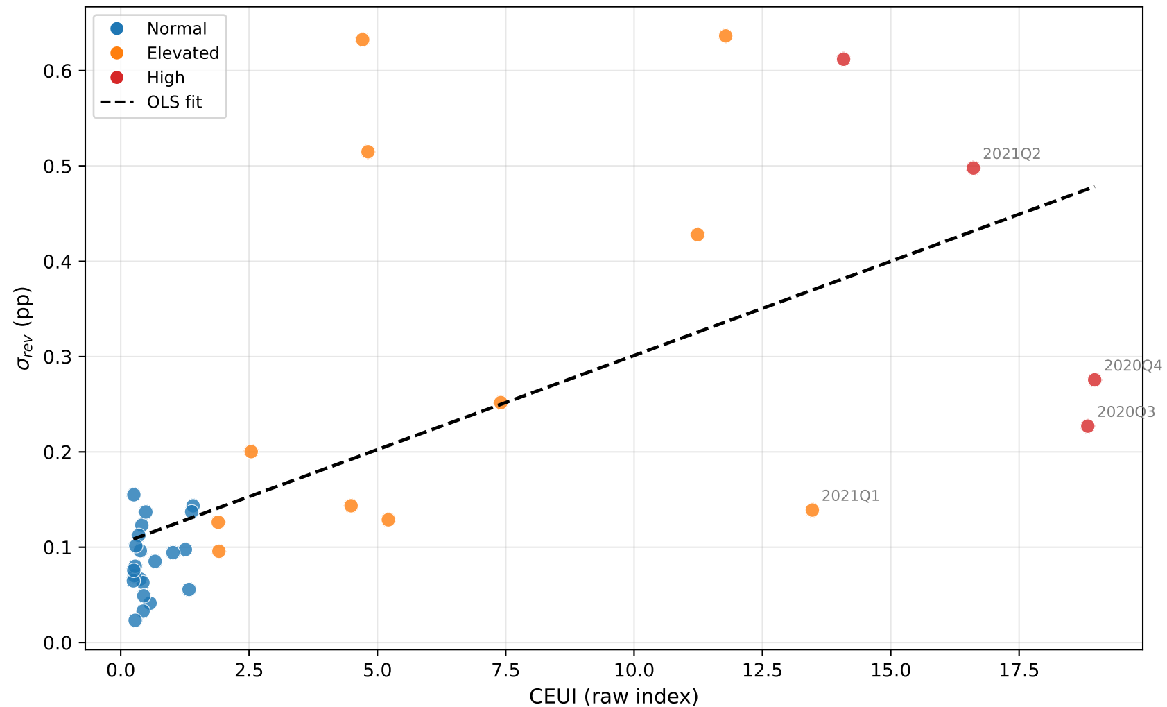
CEUI vs Revision Volatility \rho = 0.727, R^2 = 0.413, N = 37
