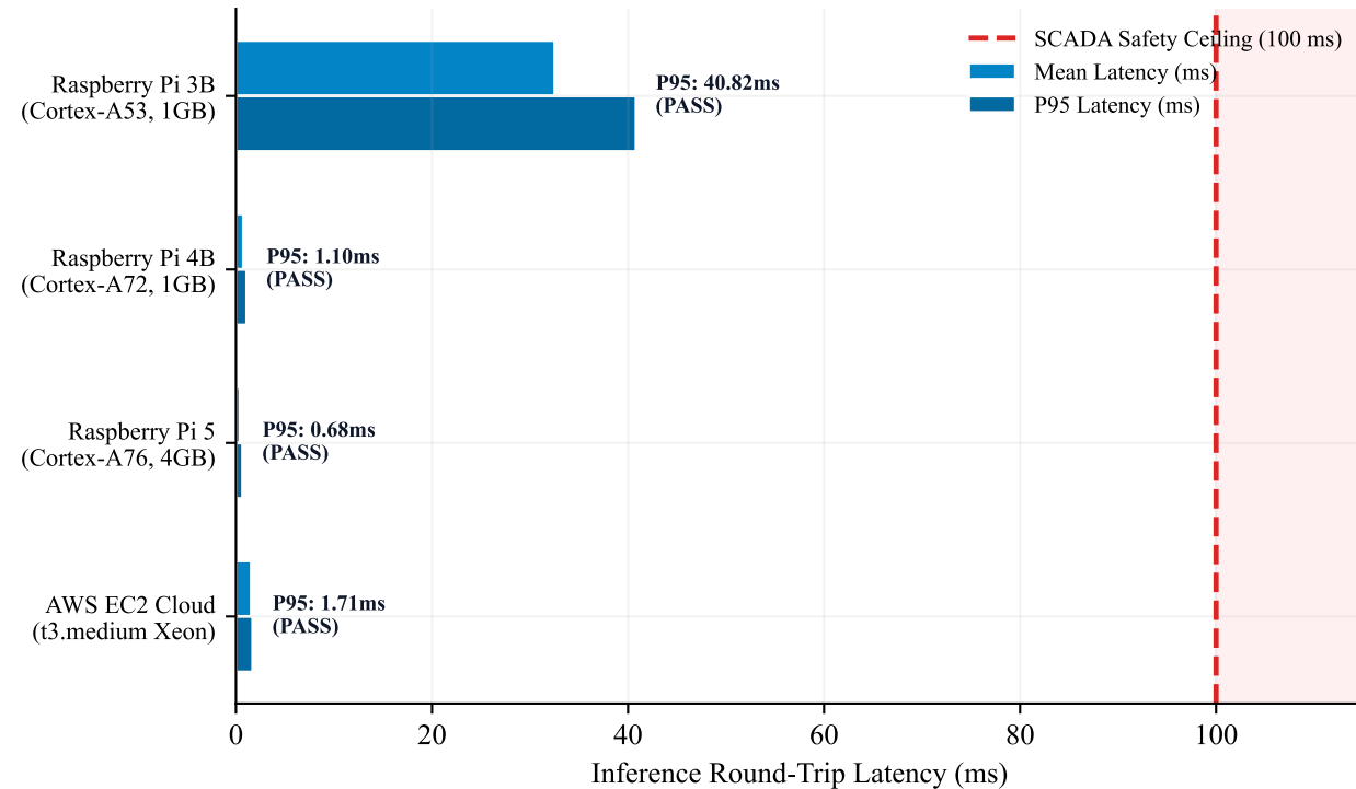
(a) Edge-to-Cloud Real-Time Inference vs SCADA Ceiling
