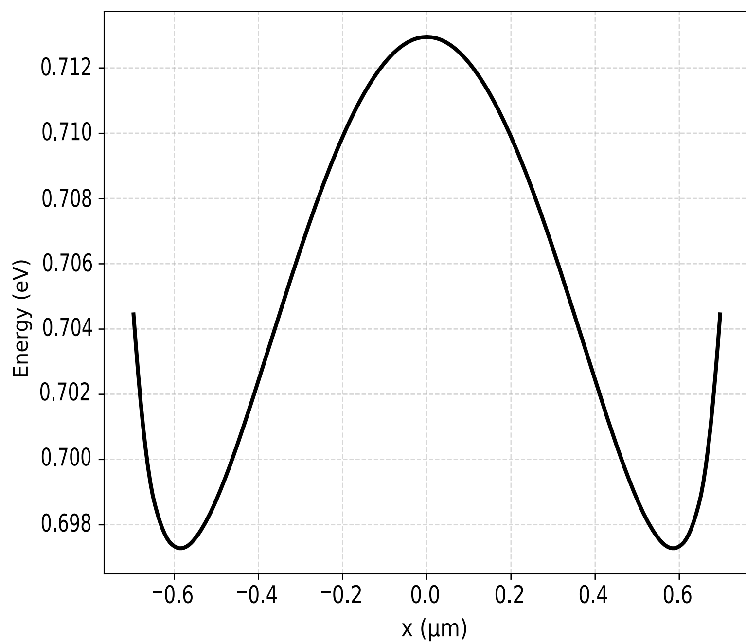
1D Double Well
