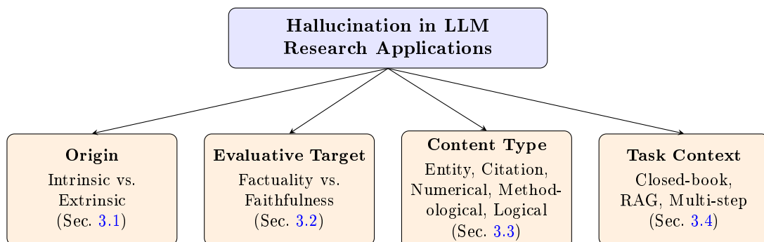
Figure 1: The four-axis taxonomy of LLM hallucination types proposed in this paper, synthesizing the origin, evaluative-target, content-type, and task-context dimensions developed in Sections 3.1–3.4.
