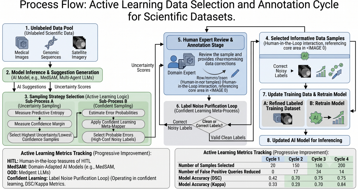
Figure 2: Process Flow of the Active Learning Data Selection and Annotation Cycle.
