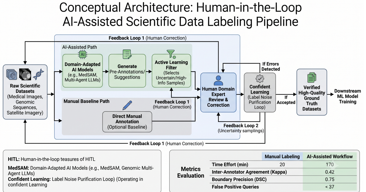
Figure 1: Conceptual Architecture of the Human-in-the-Loop AI-Assisted Scientific Data Labeling Pipeline.
