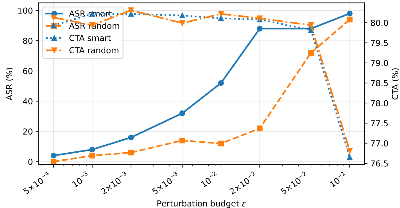
ConvNetBN, dog-bird, gradmatch
