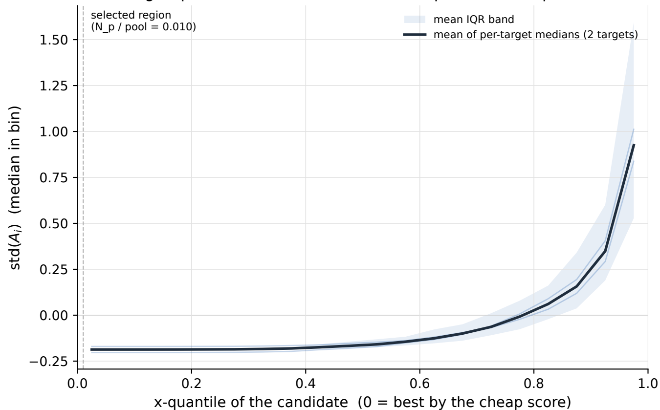
ConvNetBN / fc / frog-airplane A conditional on the cheap score (20 equal-count bins, full pool)
