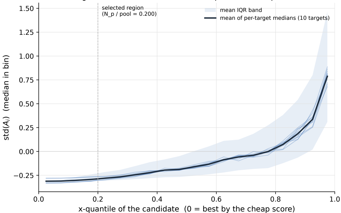
ConvNetBN / fc / dog-bird A conditional on the cheap score (20 equal-count bins, full pool)
