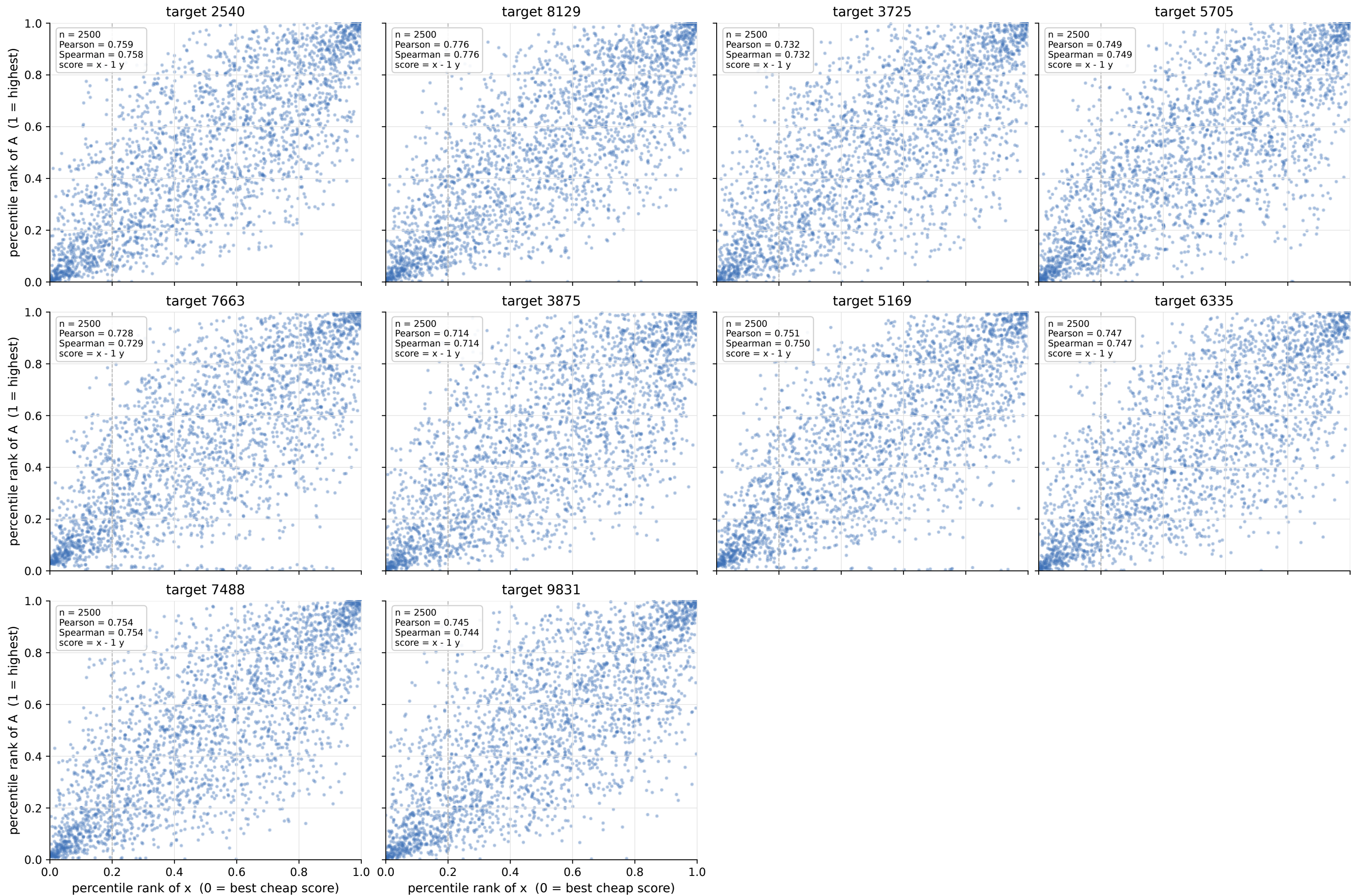
ConvNetBN / fc / dog-bird rank-rank view of the 2500 plotted candidates (dashed = N_p / pool)
