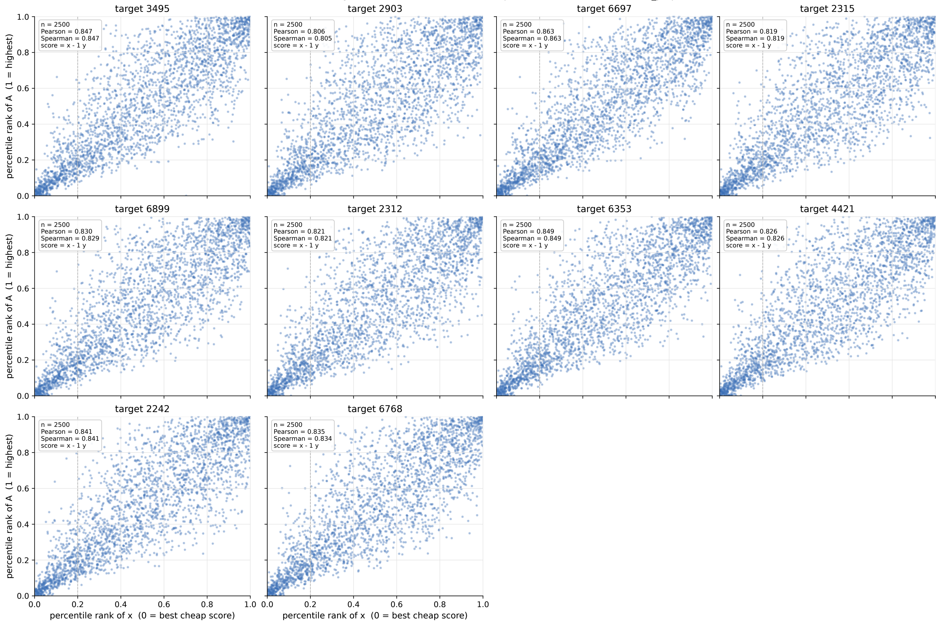
ResNet20BN / fc / dog-bird rank-rank view of the 2500 plotted candidates (dashed = N_p / pool)
