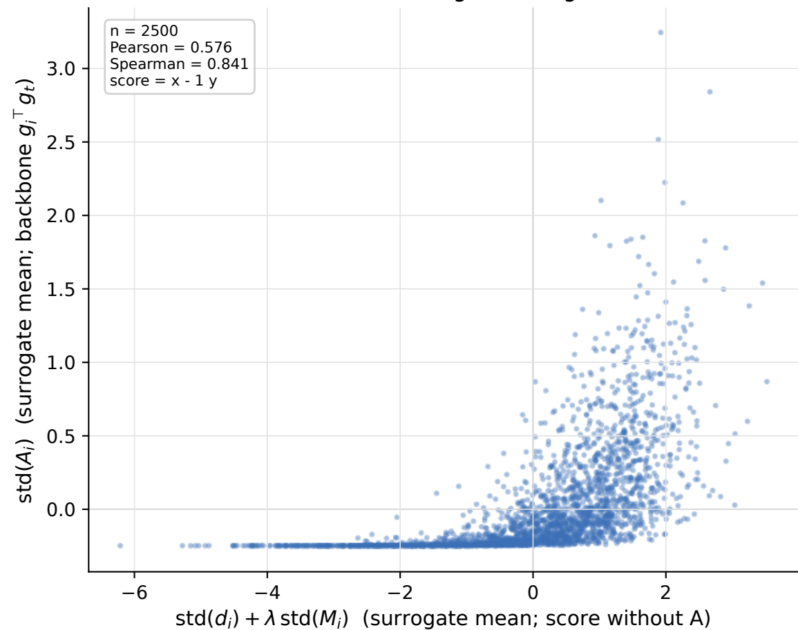
ResNet20BN / fc / dog-bird target 2242
