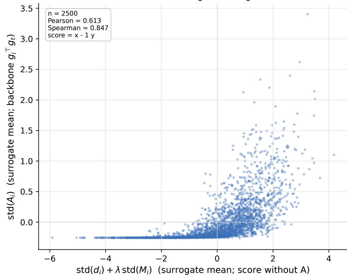
ResNet20BN / fc / dog-bird target 3495
