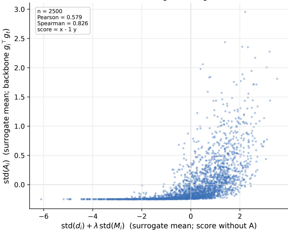
ResNet20BN / fc / dog-bird target 4421
