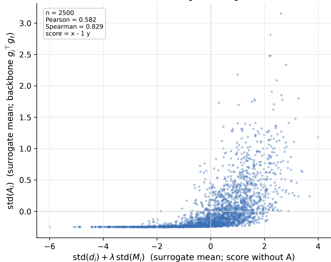
ResNet20BN / fc / dog-bird target 6899
