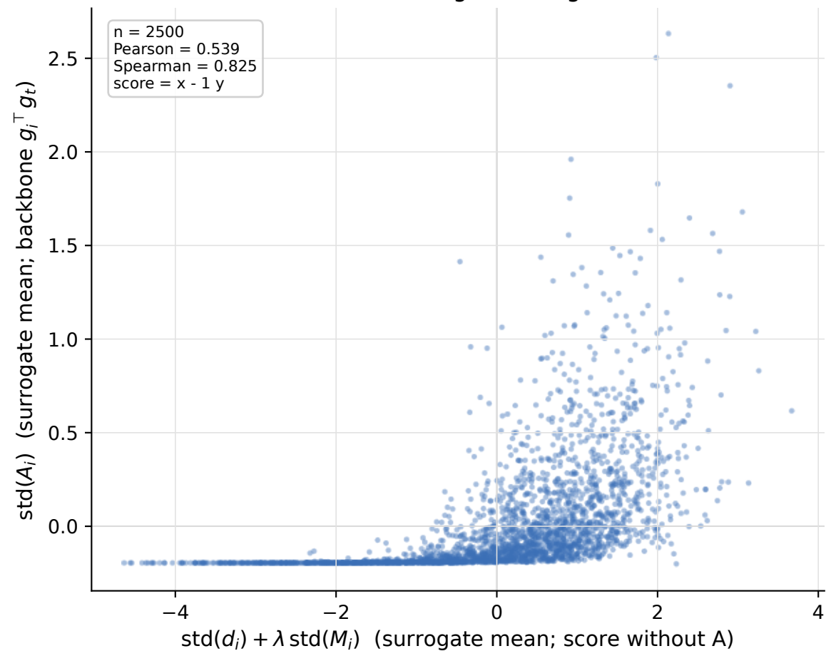
VGG13BN / fc / dog-bird target 2171
