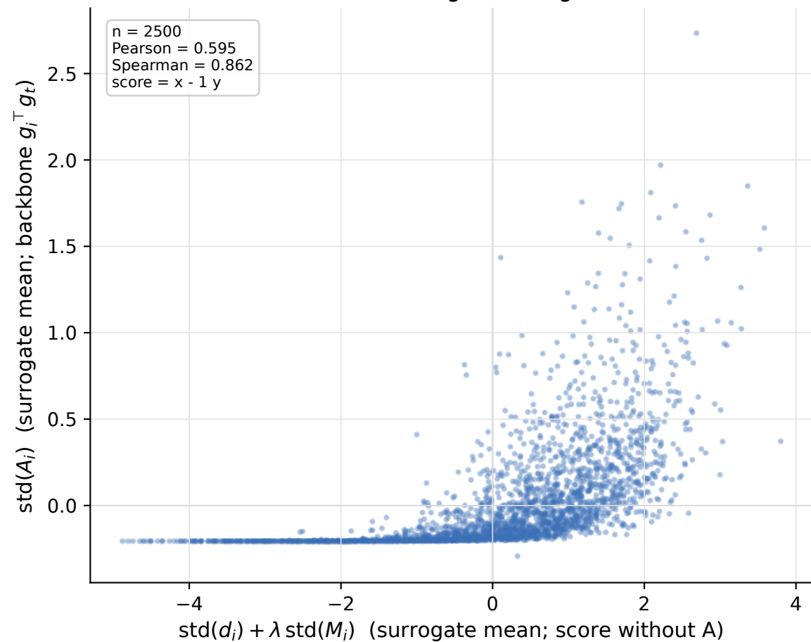
VGG13BN / fc / dog-bird target 7586
