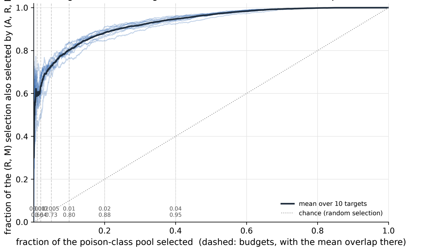
VGG13 / BN / fc / dog-bird selection agreement of (R, M) with (A, R, M) (full pool, 5000 candidates)
