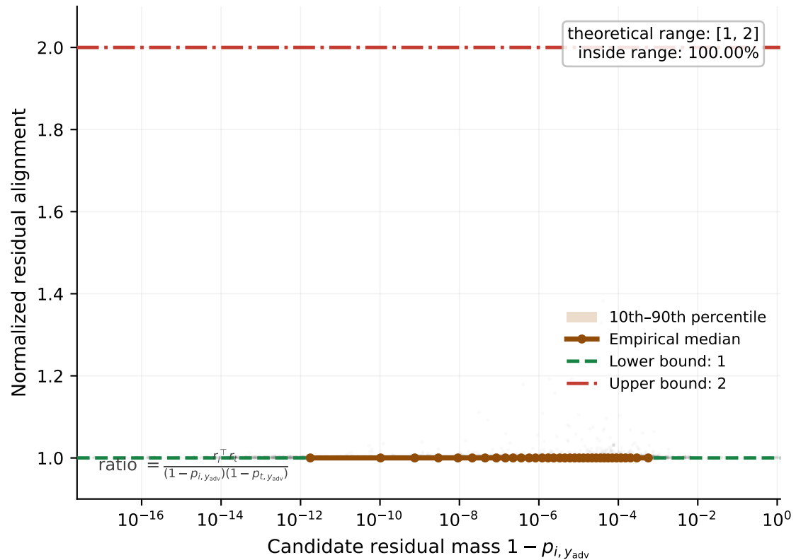
(b) Residual alignment remains within the theoretical bound
