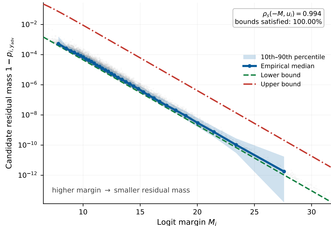
(a) Margin predicts residual magnitude
