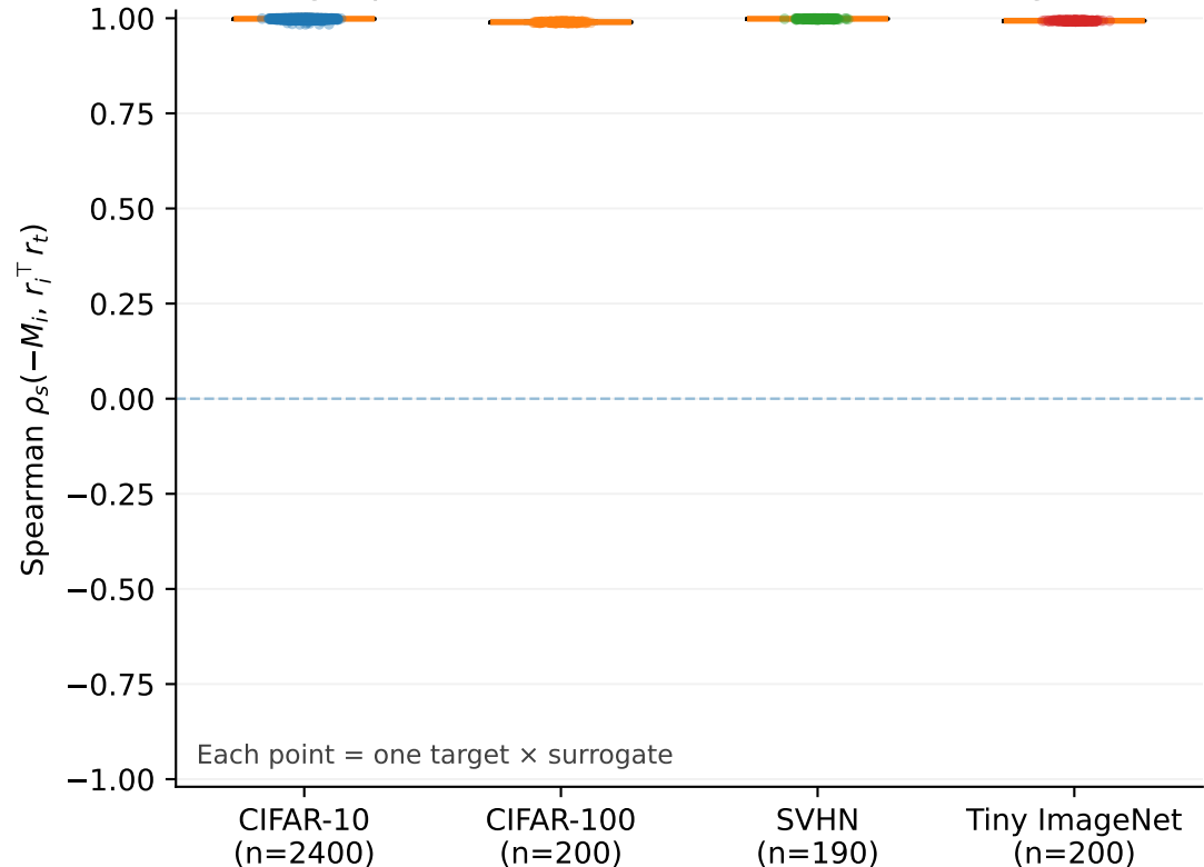
(b) Margin preserves residual-interaction ranking
