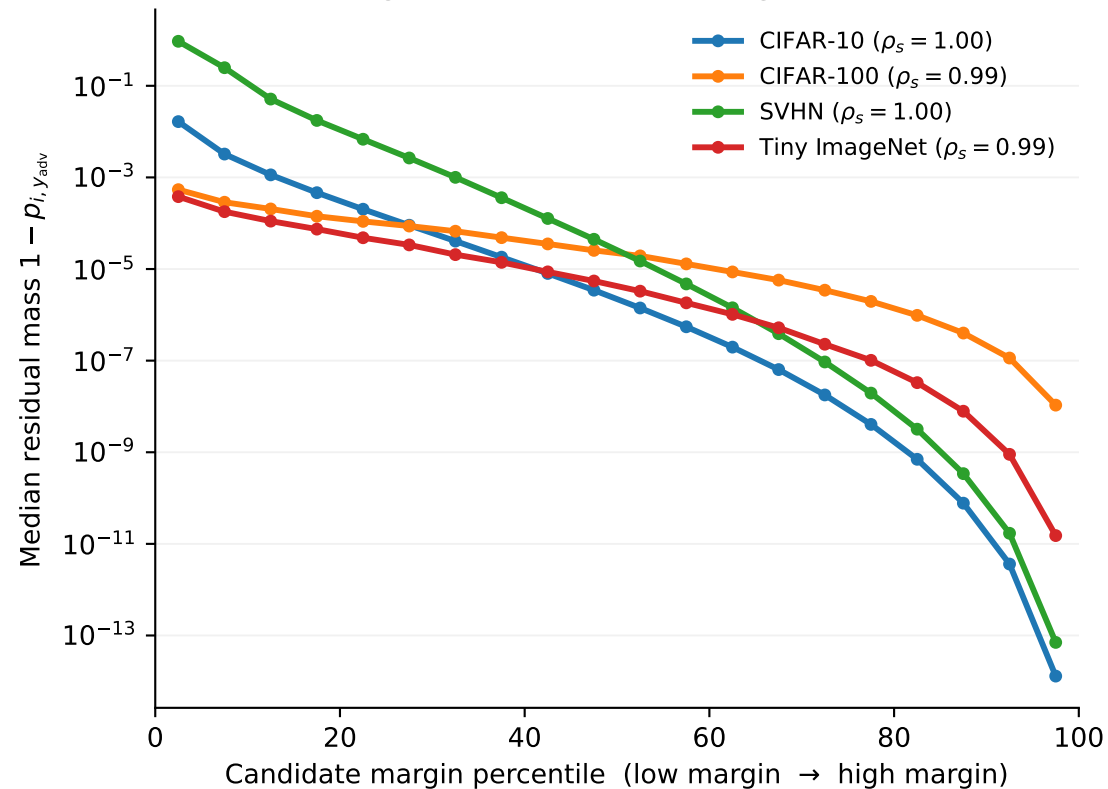
(a) Lower-margin candidates have larger residuals
