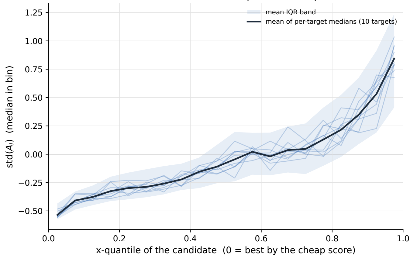
ConvNetBN / fc / 3-7 A conditional on the cheap score (20 equal-count bins, full pool)
