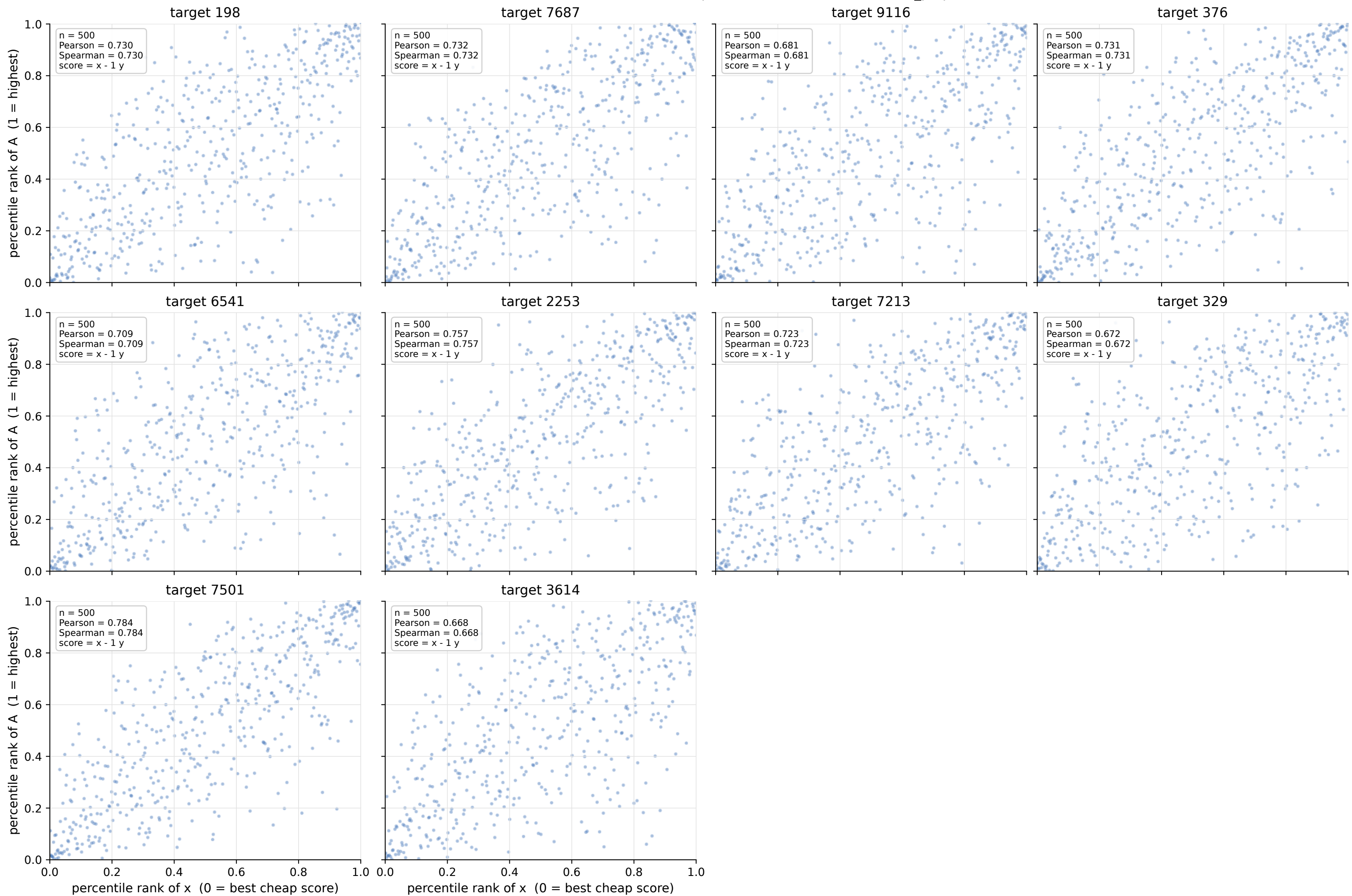
ConvNetBN / fc / 3-7 rank-rank view of the 500 plotted candidates (dashed = N p / pool)
