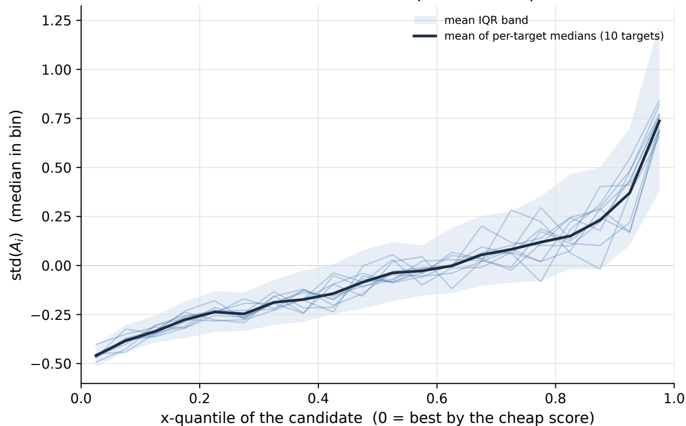
ResNet20BN / fc / 3-7 A conditional on the cheap score (20 equal-count bins, full pool)
