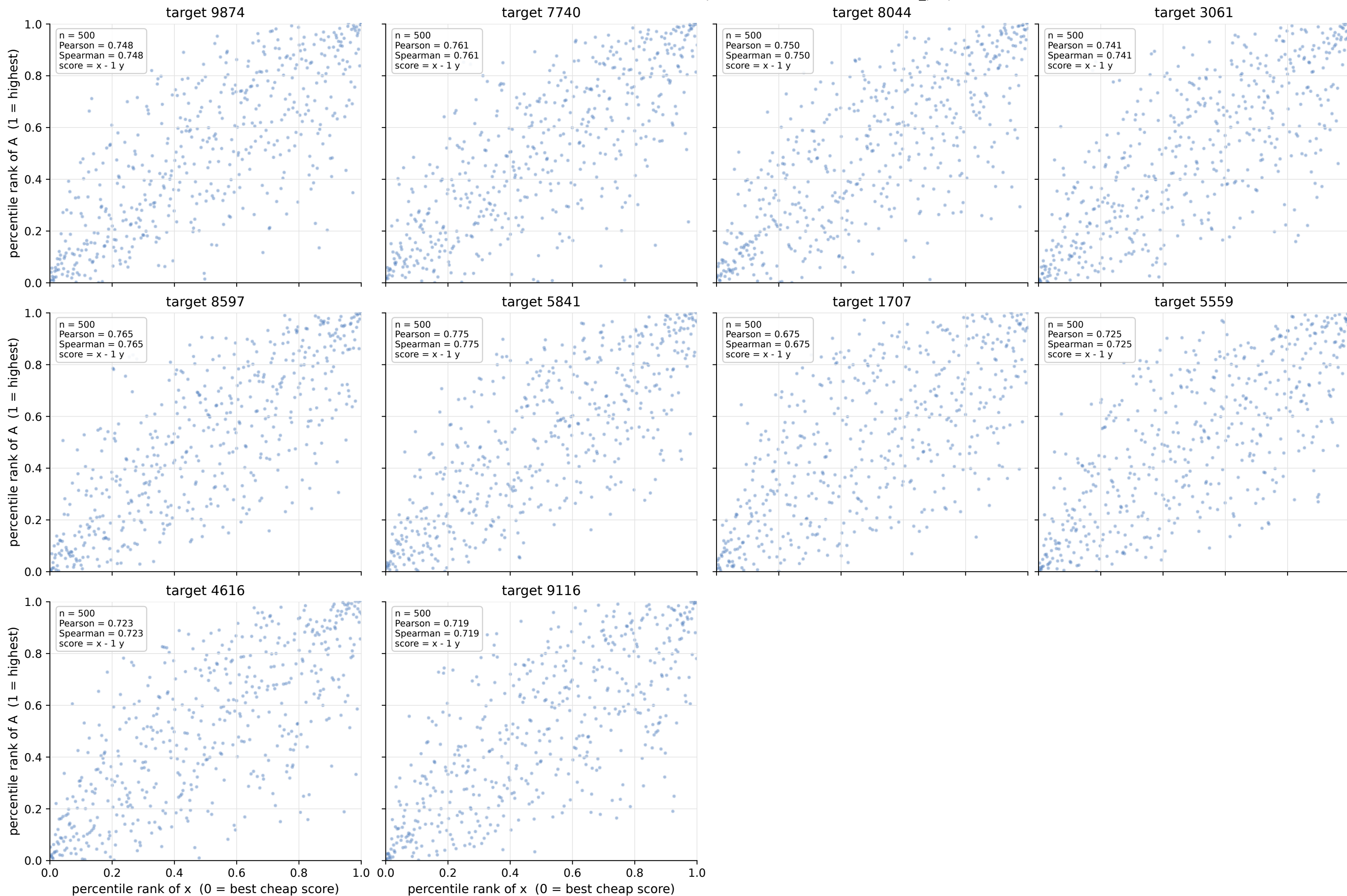
ResNet20BN / fc / 3-7 rank-rank view of the 500 plotted candidates (dashed = N p / pool)
