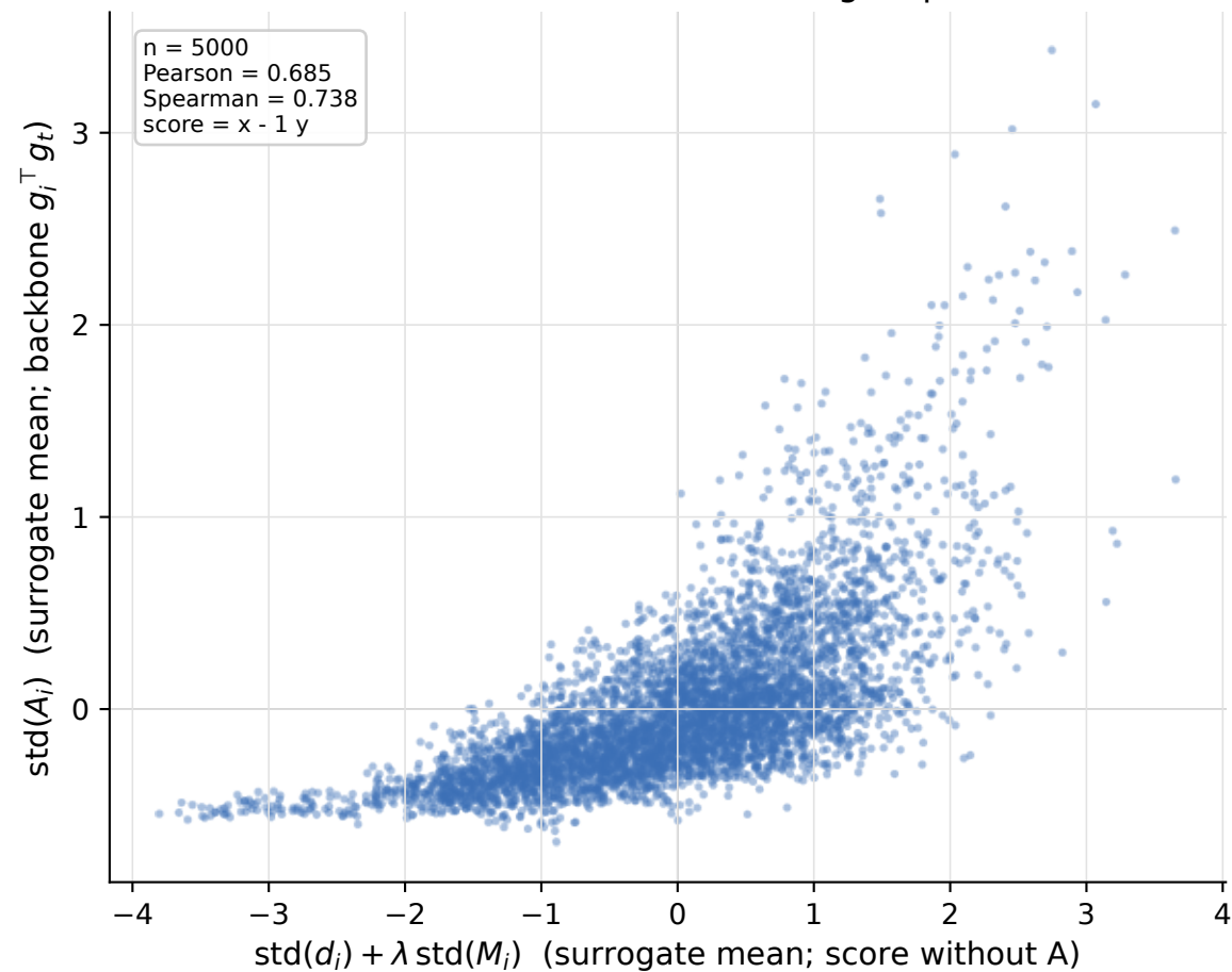
ResNet20BN / fc / 3-7 all 10 targets pooled
