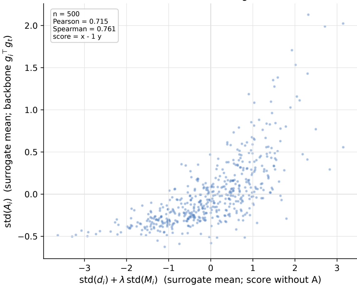
ResNet20BN / fc / 3-7 target 7740
