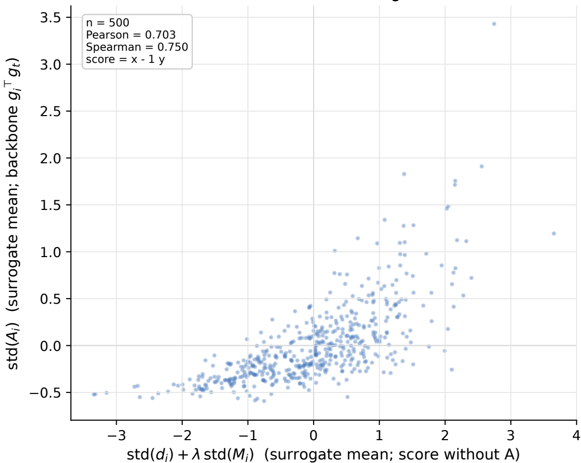
ResNet20BN / fc / 3-7 target 8044
