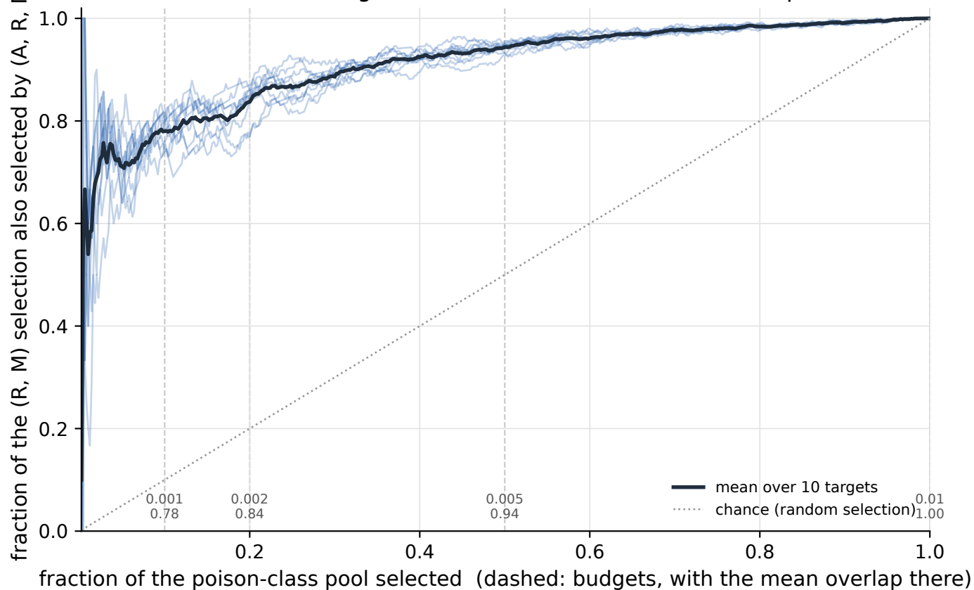
ResNet20BN / fc / 3-7 selection agreement of (R, M) with (A, R, M) (full pool, 500 candidates)
