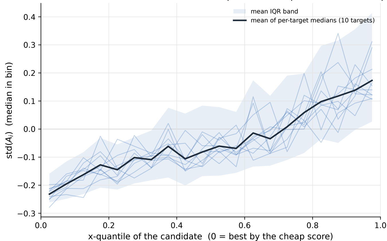
VGG13BN / fc / 3-7 A conditional on the cheap score (20 equal-count bins, full pool)
