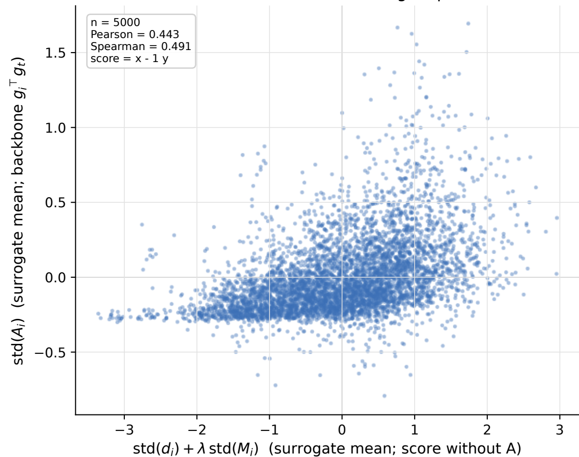
VGG13BN / fc / 3-7 all 10 targets pooled
