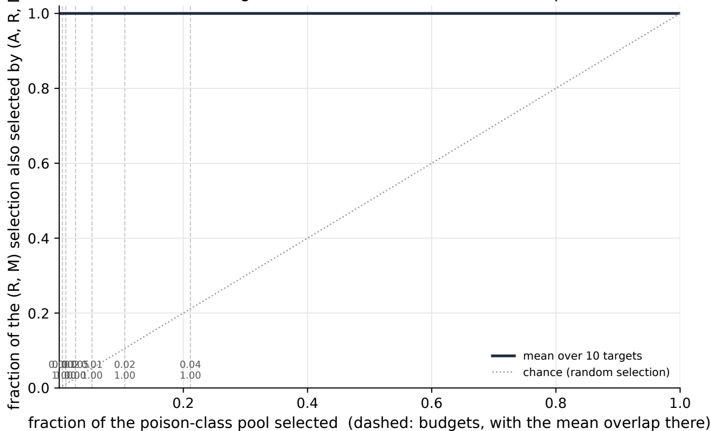
VG-13BN / fc / 1-7 selection agreement of (R, M) with (A, R, M) (full pool, 13861 candidates)
