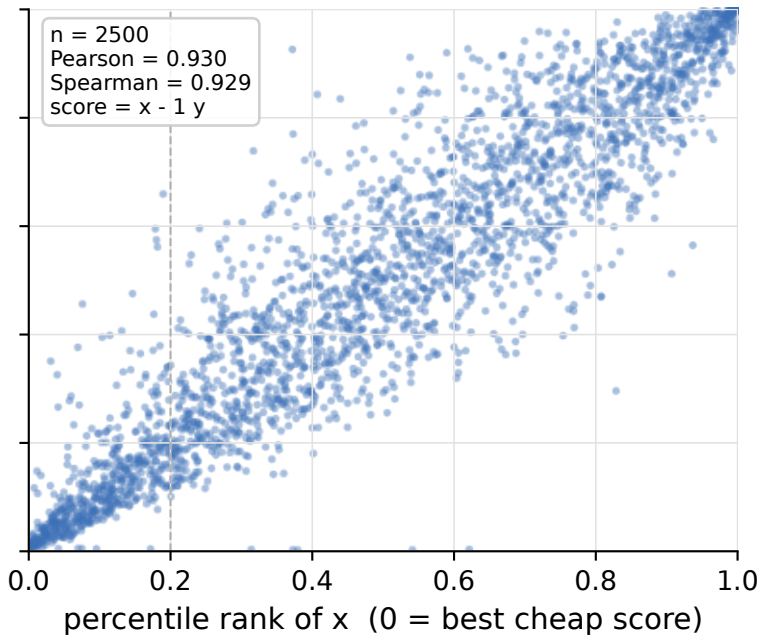
ConvNetBN / fc / dog-bird rank-rank view of the 2500 plotted candidates (dashed = N_p / pool) target 2540
