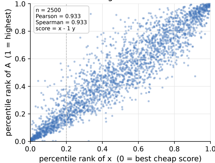
ConvNetBN / fc / dog-bird rank-rank view of the 2500 plotted candidates (dashed = N_p / pool) target 2540
