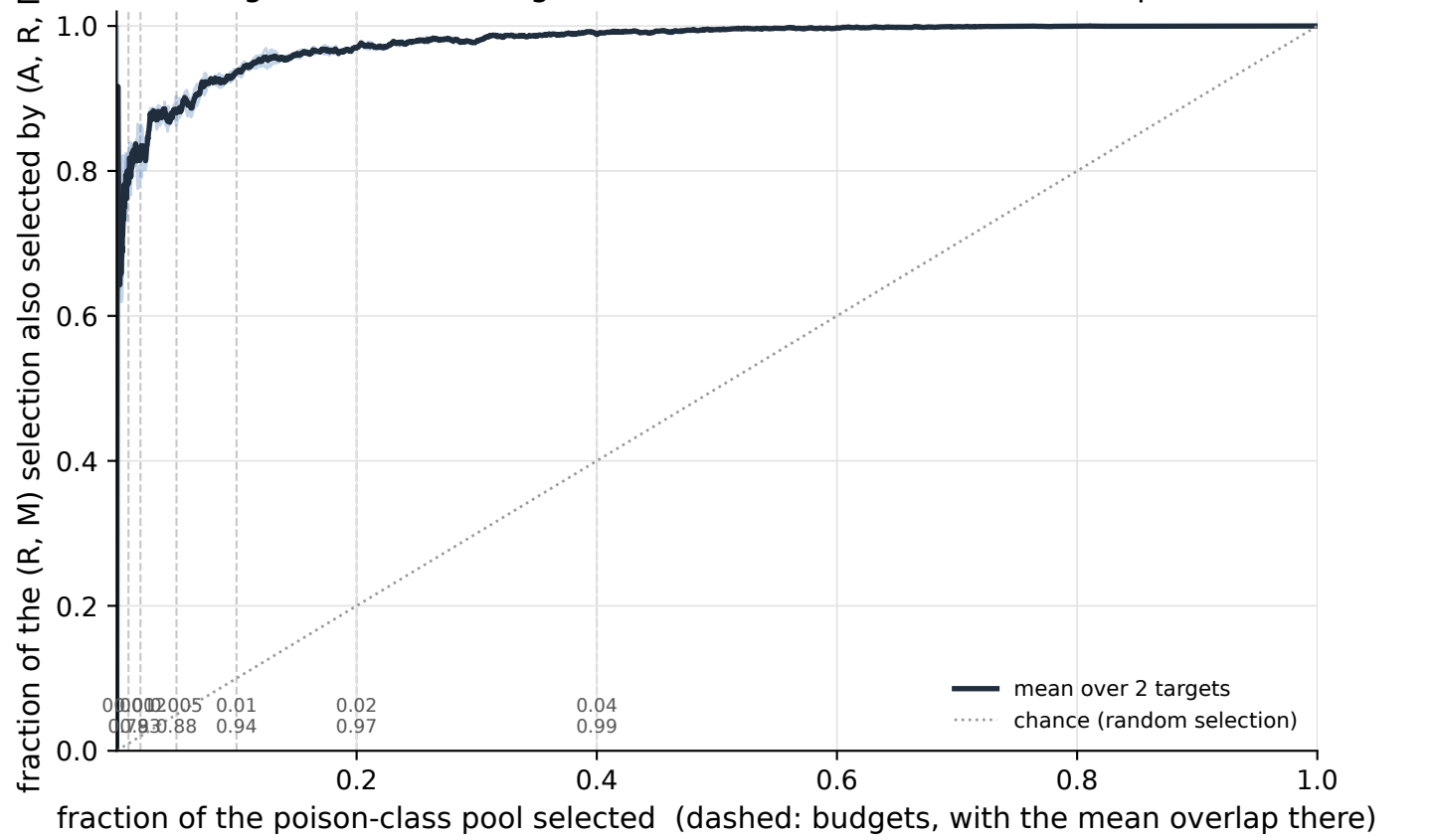
ConvNetBN / fc / dog-bird selection agreement of (R, M) with (A, R, M) (full pool, 5000 candidates)
